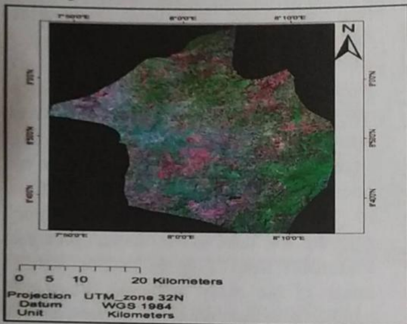
Figure 2: RGB colour composite of study area in Bands 7, 4 and 2 respectively.
