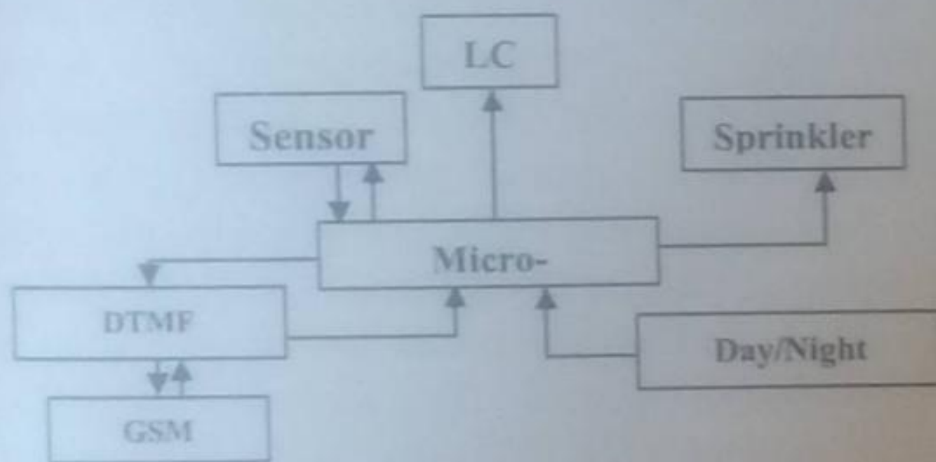
Figure 1: Block diagram of the irrigation control system.
