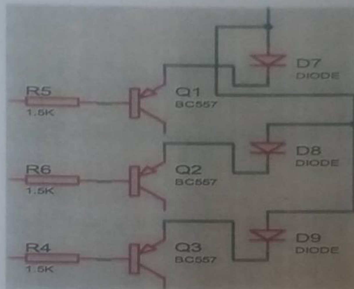
Figure 4: Phone Transistors Driver
