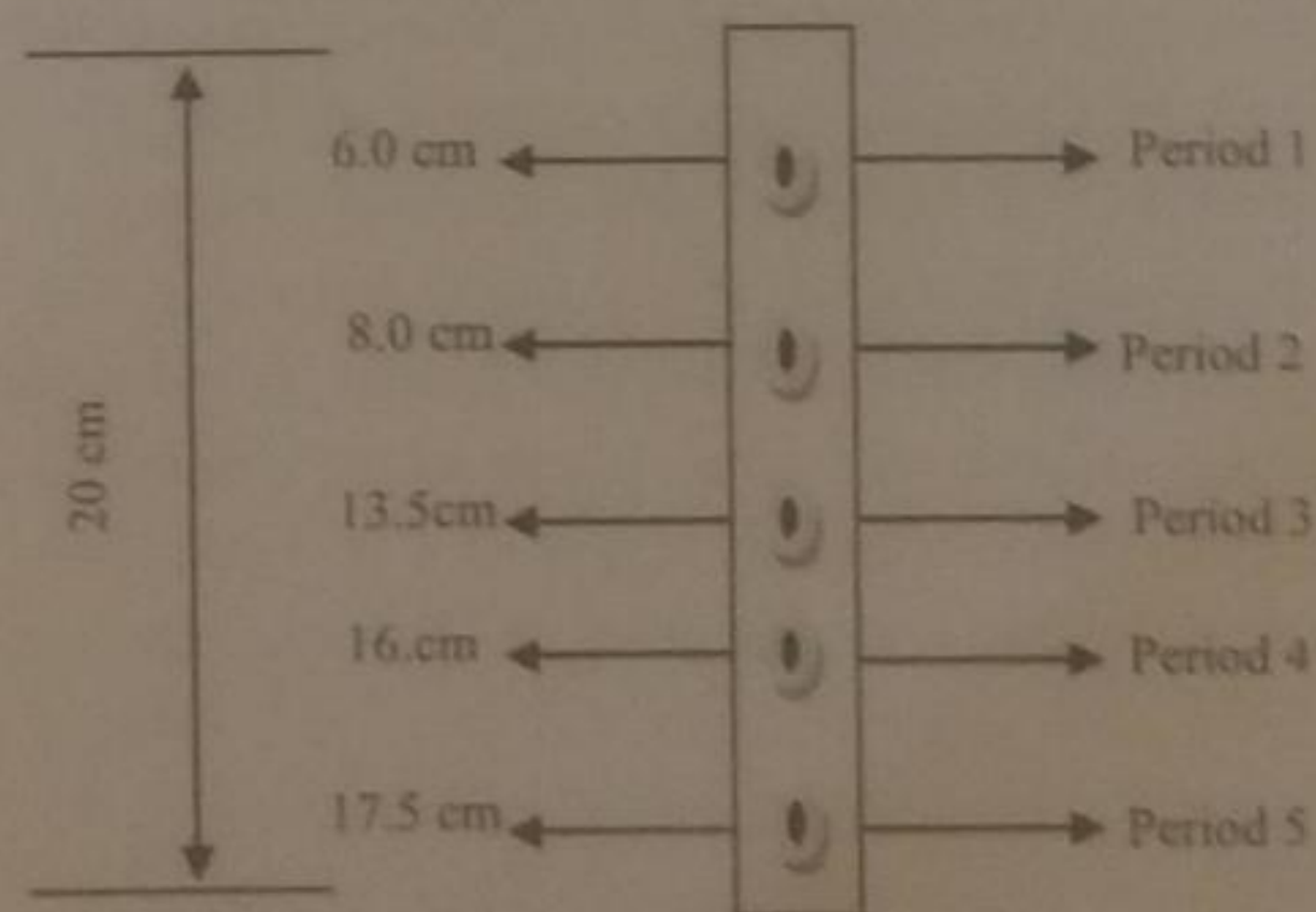
Figure 2: Calibration of Sensor
