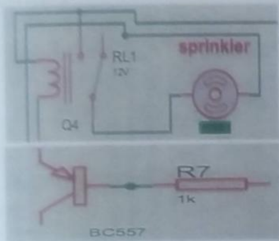
Figure 6: The Sprinkler Section.
