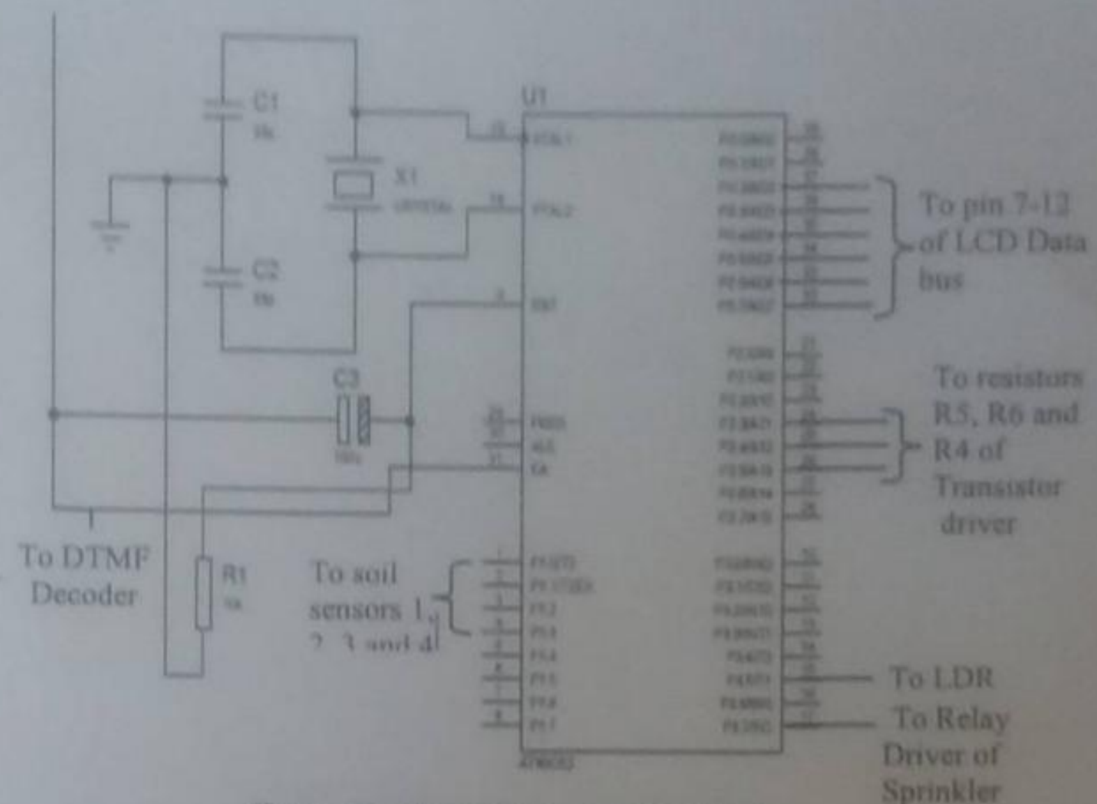
Figure 3: The Microcontroller Unit
