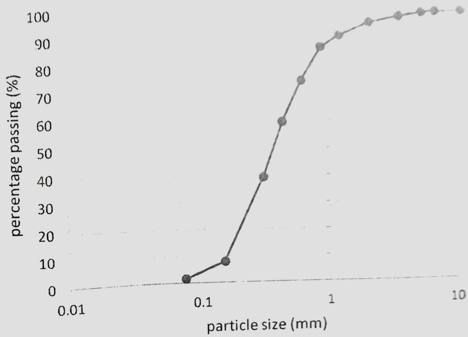
Figure 1 Sieve analysis of fine aggregate
