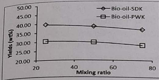
Fig. 6: Effect of mixing ration on bio-oil yield at 500°C.
