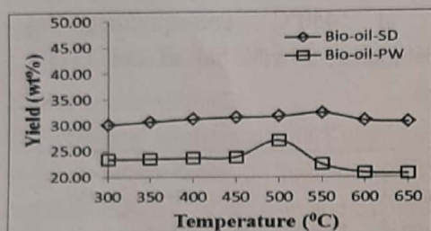
Fig. 3: Effect of temperature on bio-oil yields.
