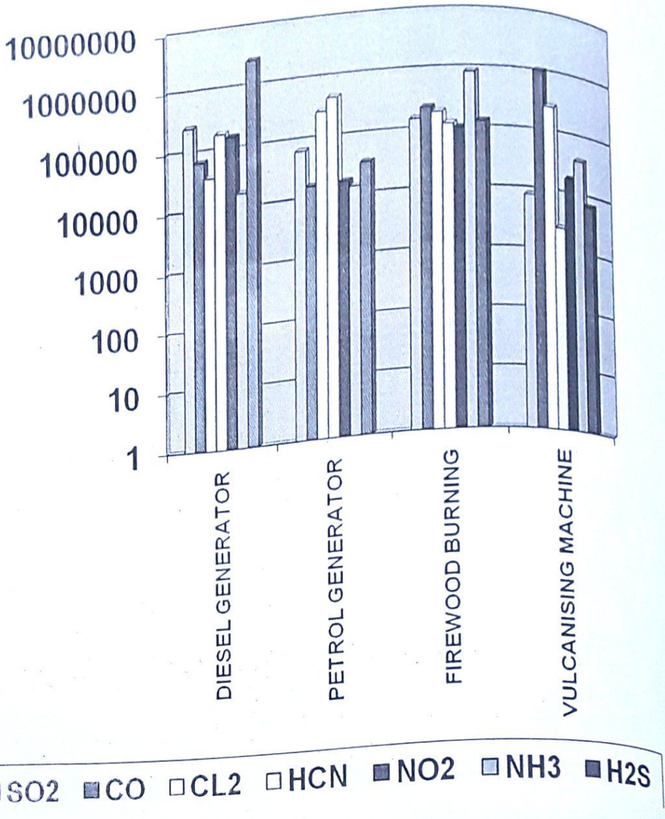
Fig.2. Bar Chart Representation of the Sources of Pollution: Lagos/Kaduna Road neighbourhood (vertical scale in \mu\text{g}/\text{m}^3 )
