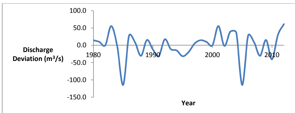
Fig. 2. Discharge deviation
