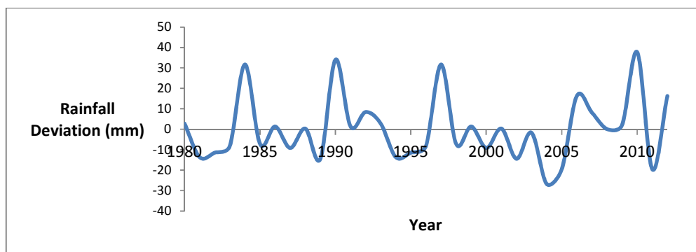
Fig. 4. Rainfall Deviation
