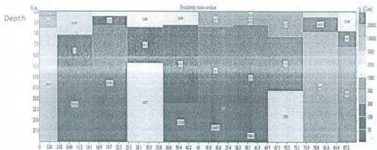
Figure 3d: Goelectric Section for Tranverse D
