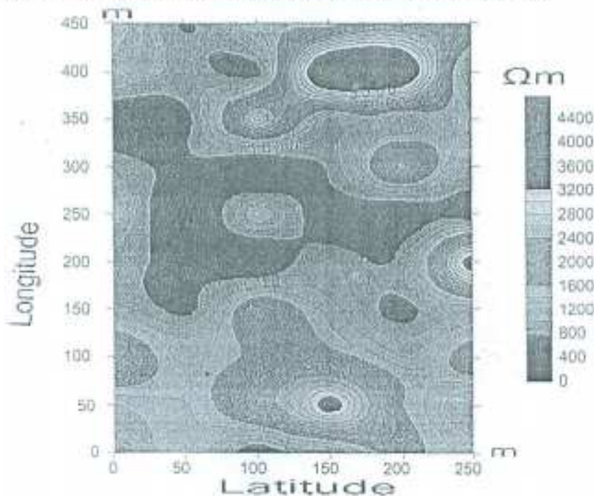
Figure 4 a: Iso-resistivity Map at First Layer
