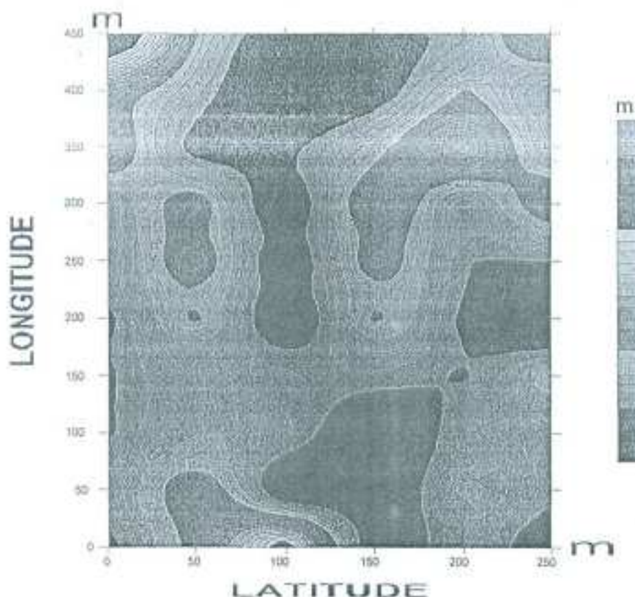
Figure 5: Depth to Basement Map of the Area
