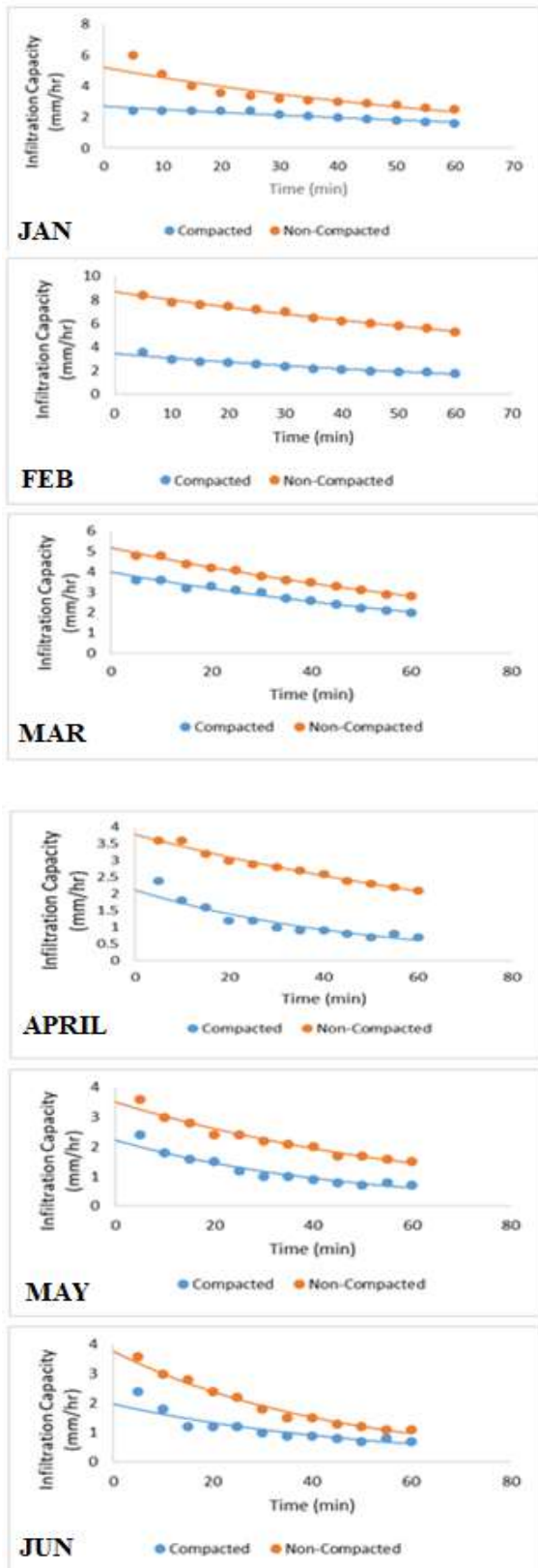
Fig. 5: Infiltration rates (Jan-June) for compacted and non-compacted soil for Station 3 (dry & wet season)
