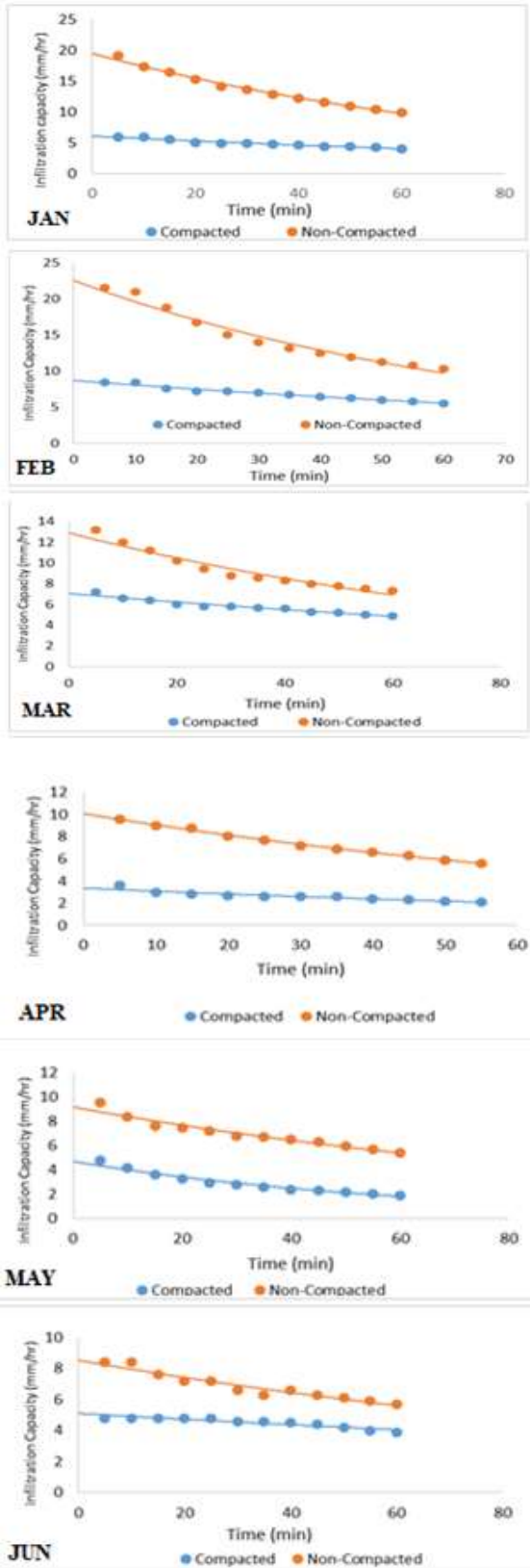
Fig. 3: Infiltration rates (Jan-June) for compacted and non-compacted soil for Station 1 (dry & wet season)
