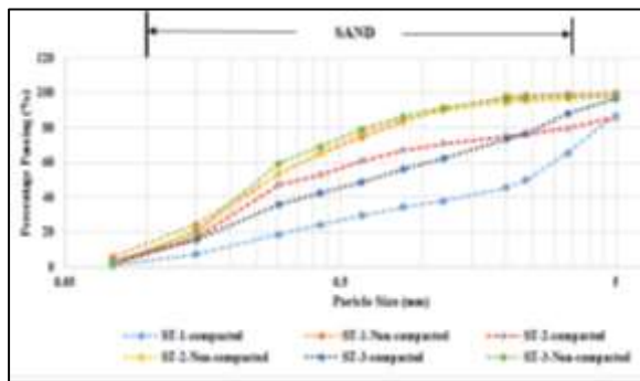
Fig. 2: Particle size distribution of Compacted and Non-compacted soil in all Stations
