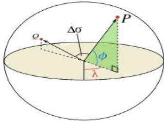
FIGURE 7. An illustration of the central angle, Δσ, between two points, P and Q (longitudinal (λ) and latitudinal (φ) angles of P respectively).
