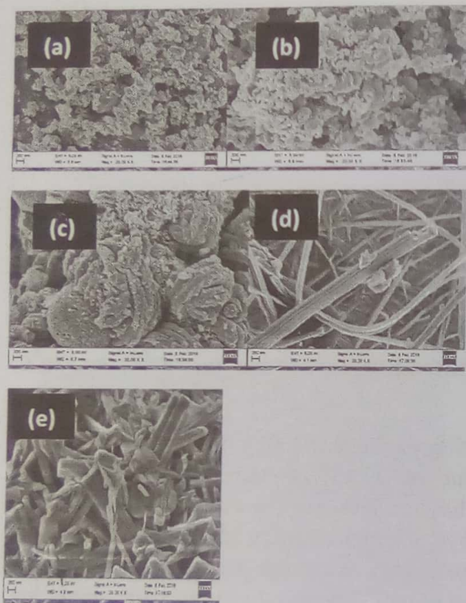
Figure 3: HRSEM micrograph of (a) undoped \text{WO}_3 (b) Boron (c) Aluminium (d) Phosphorus (e) Iodine doped \text{WO}_3 nanoparticles
