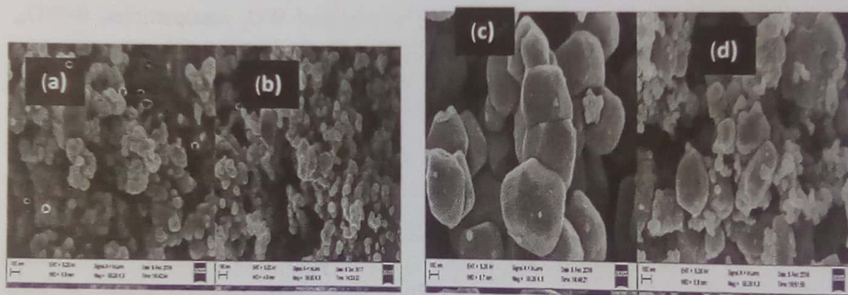
Figure 1: HRSEM micrograph of WO 3 nanoparticles synthesised at (a) 450°C (b) 550°C (c) 650°C (d) 750°C
