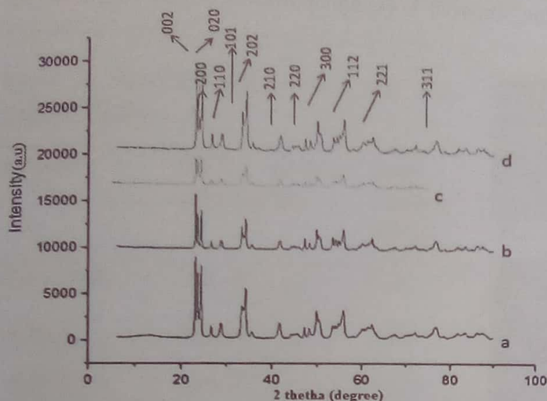
Figure 2: XRD pattern of \text{WO}_3 prepared at different temperatures (a) 450^\circ\text{C} (b) 550^\circ\text{C} (c) 650^\circ\text{C} (d) 750^\circ\text{C}
