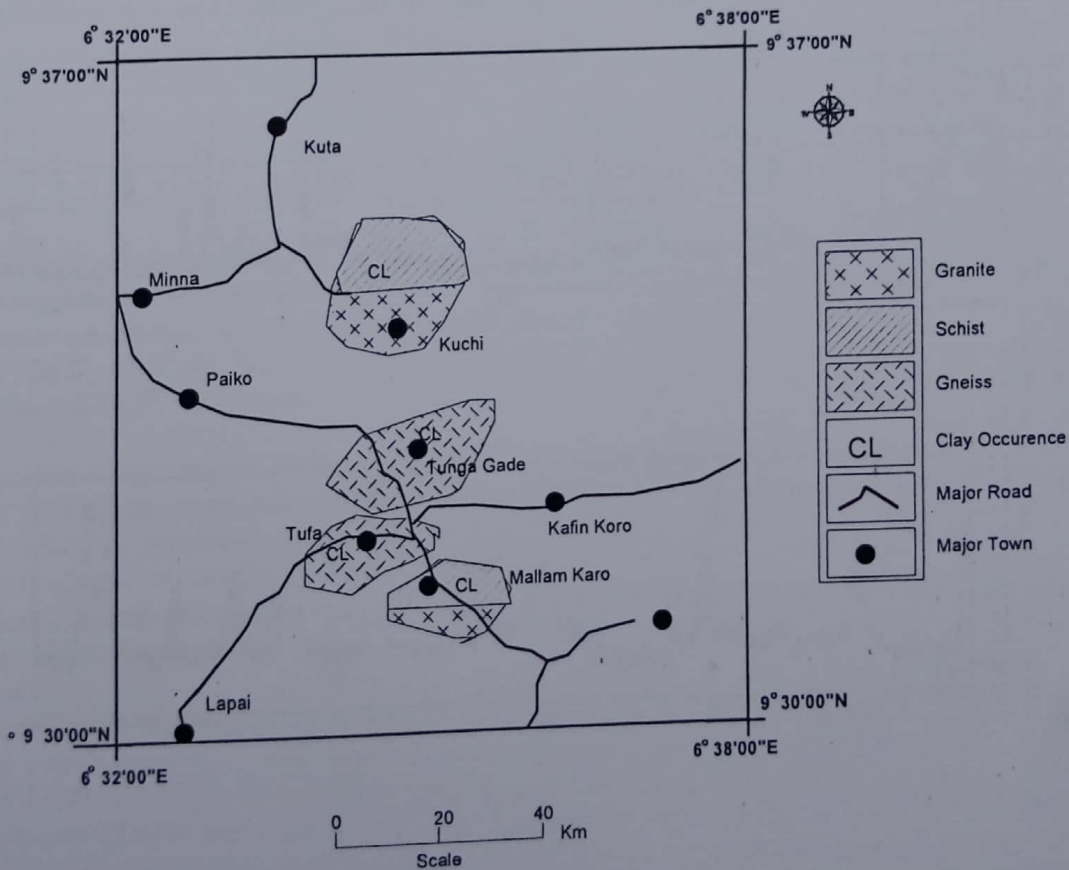
Fig 2 : Geological Map of the Study area and Clay site
