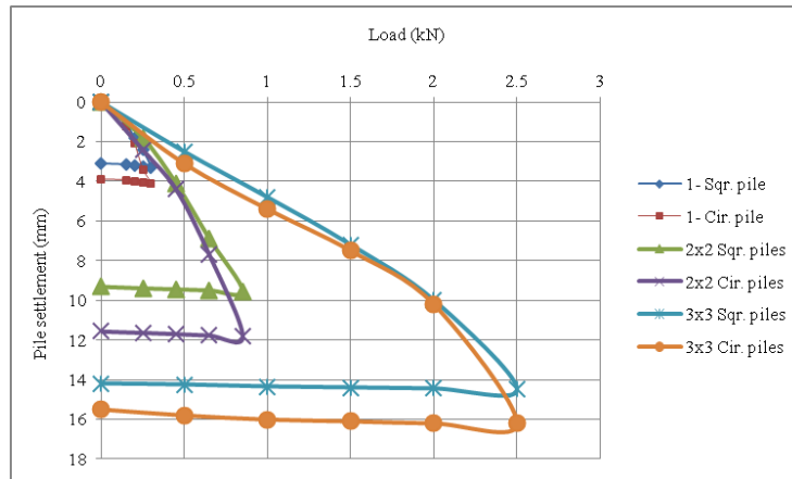
Fig. 6 Load – Settlement Curve for Loading rate 0.1 mm/min
