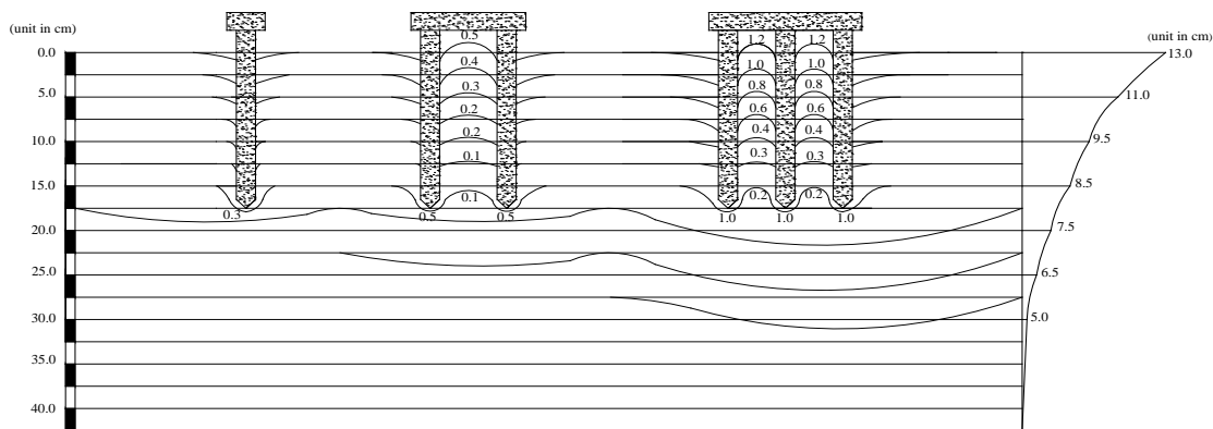
Fig. 10 Deformation of Soils around Circular Piles under Load
