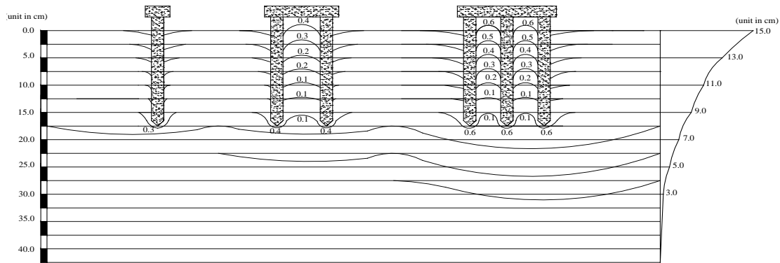
Fig. 9 Deformation of Soils around Square Piles under Load
