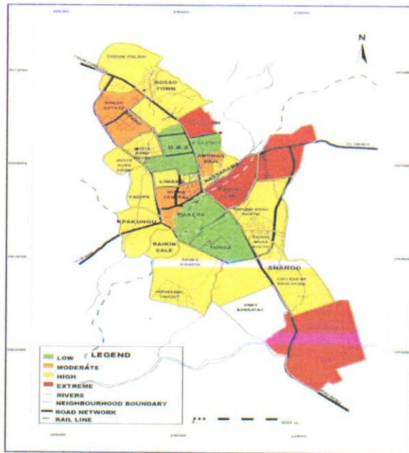
Figure 4: Flood Hazard Probability and Risk Levels in Minna Source: Authors' Analysis, 2013.
