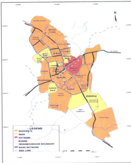
Figure 3: Rainstorm Hazard Probability and Risk Levels in Minna
