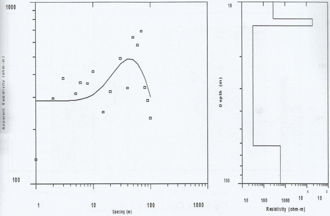
Fig. 4: AK curve of VES 23
