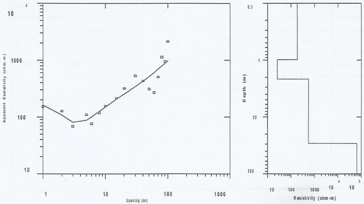
Fig. 6: HA Curve of VES 48
