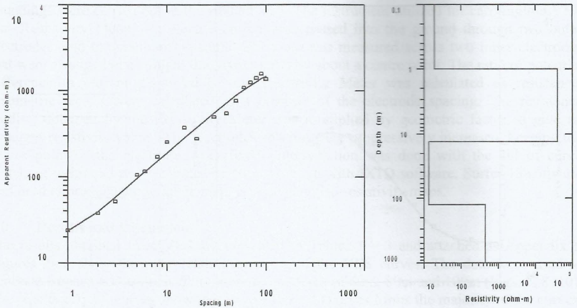
Fig. 5: A curve of VES 22
