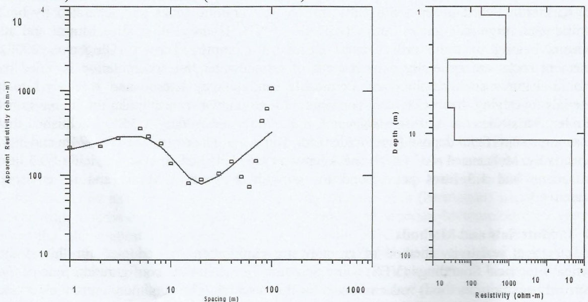
Fig. 2: A Curve of VES 2
