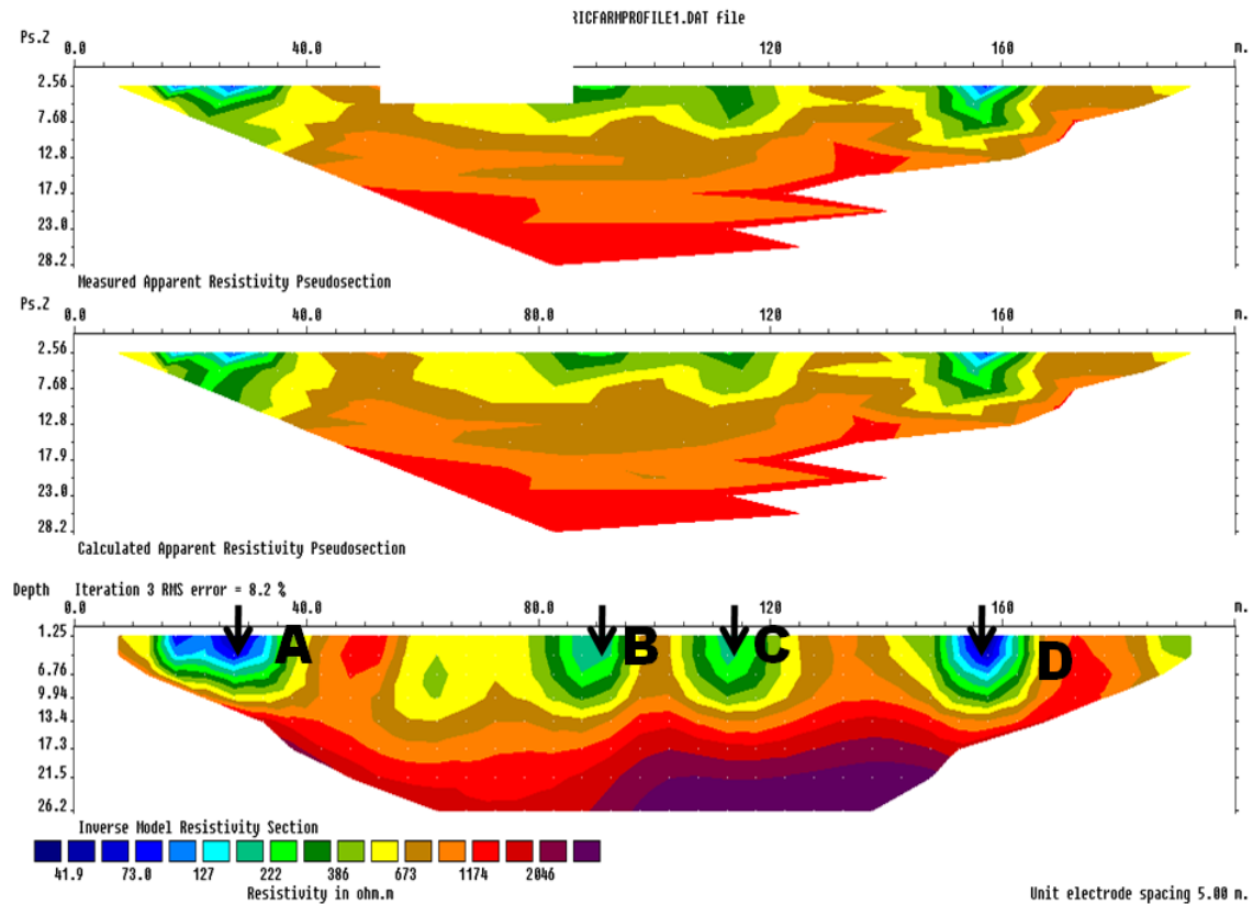
Figure 3: Result of 2-D inversion of the Wenner-array data along profile 1
