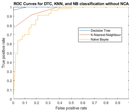
Fig. 5. ROC Curves for DTC, KNN, and NB classifiers trained without NCA selected features of non-post-processed images.
