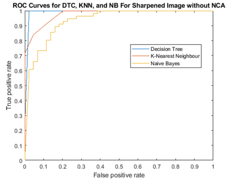
Fig. 4. ROC Curves for DTC, KNN, and NB classifiers trained without NCA selected features of post-processed images.
