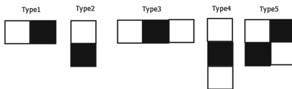
Fig. 2. Haar features in Viola Jones
