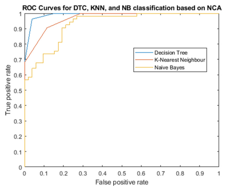
Fig. 6. ROC Curves for DTC, KNN, and NB classifiers trained with NCA selected features of non-post-processed images.
