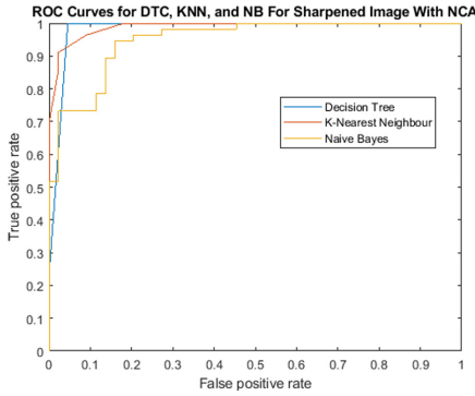
Fig. 3. ROC Curves for DTC, KNN, and NB classifiers trained with NCA selected features of post-processed images.
