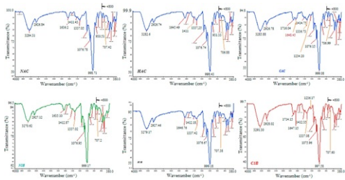
Fig. 3 FTIR of native and modified acha and iburu starches. (NAC: native acha starch; HAC: heat moisture treated acha starch; CAC: citric acid modified acha starch; NIB: native iburu starch; HIB: heat moisture treated iburu starch; CIB: citric acid modified iburu starch).
