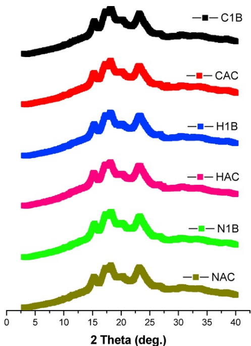
Fig. 2 X-ray diffraction of native and modified starches (NAC: native acha starch; HAC: heat moisture treated acha starch; CAC: citric acid modified acha starch; NIB: native iburu starch; HIB: heat moisture treated iburu starch; CIB: citric acid modified iburu starch).
