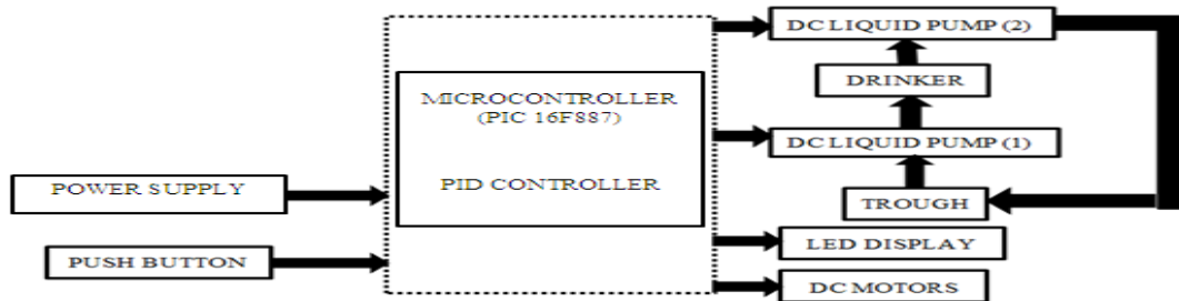
Figure 2: Block diagram of the Proposed Design
