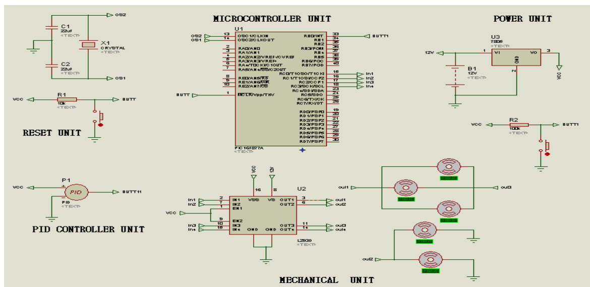
Figure 3: Electronic circuit diagram of Proposed System
