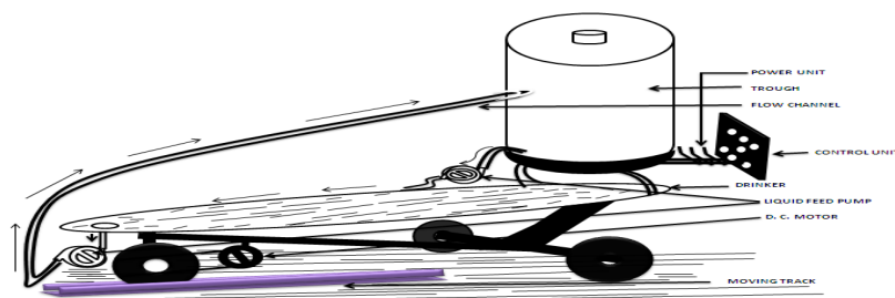
Figure 1: Schematic of the Mobile poultry liquid feed dispensing system.
