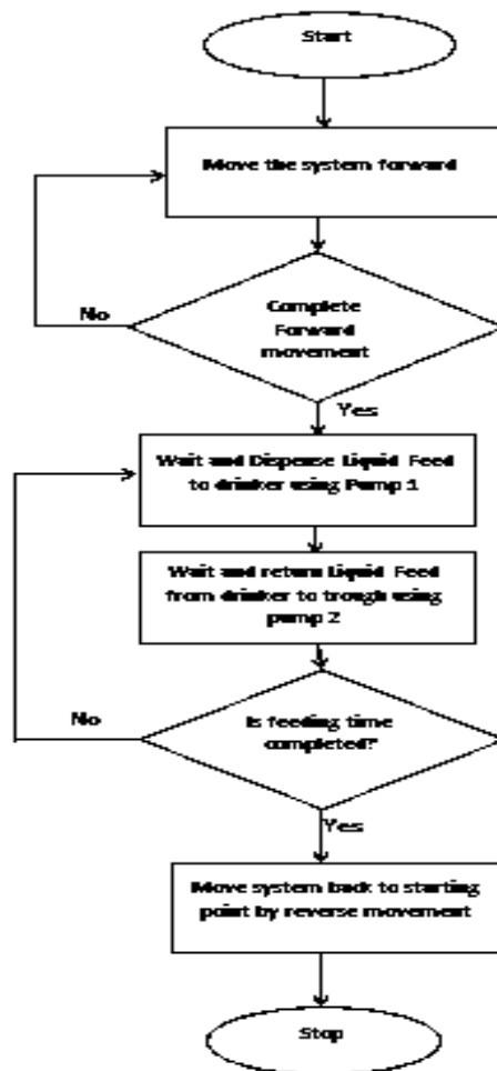
Figure 4: Flowchart diagram of mobile poultry liquid feed dispensing system
