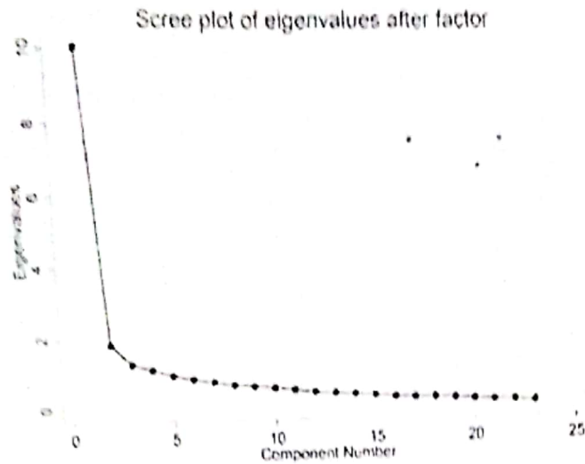
Figure 5. Catell's scree test
