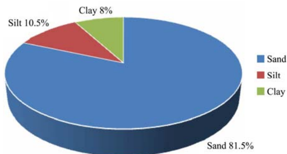
Figure 2 Soil textural classes
