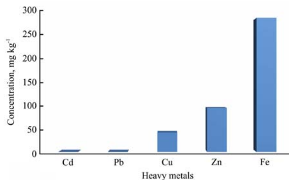
Figure 3 Heavy metals concentration in the soil sample
