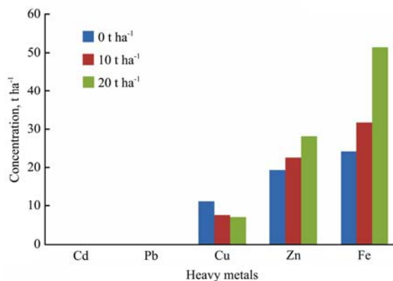
Figure 5 Heavy metals in the okra fruit grown with different sewage sludge rate
