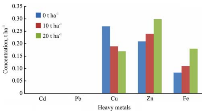
Figure 6 Transfer factors of heavy metals in okra fruit grown with different sewage sludge application rate
