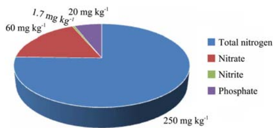
Figure 4 Chemical composition of sewage sludge
