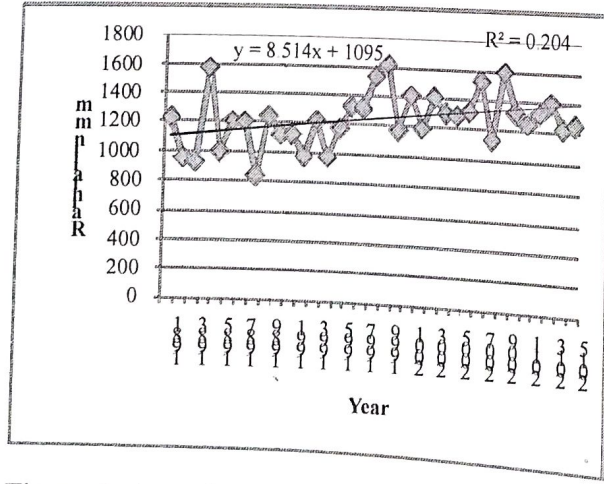
Figure 6: Annual rainfall over Lafia, 1981–2015 Figure 7: Annual rainfall over Abuja, 1983–2015 Source: Authors' computation, 2018 Source: Authors' computation, 2018
