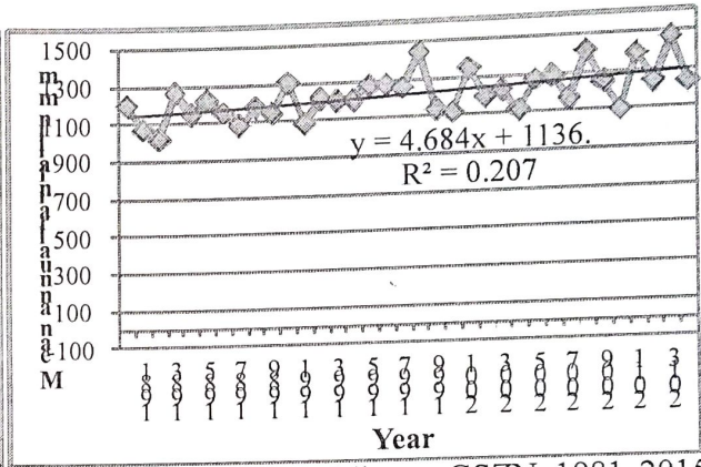
Figure 11: Mean annual rainfall over GSZN, 1981-2015 Source: Authors' computation, 2018
