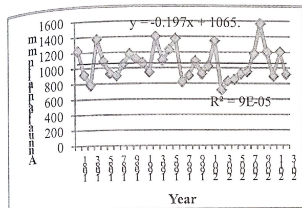
Figure 10: Annual rainfall over Ibi, 1981-2013 Source: Authors' computation, 2018
