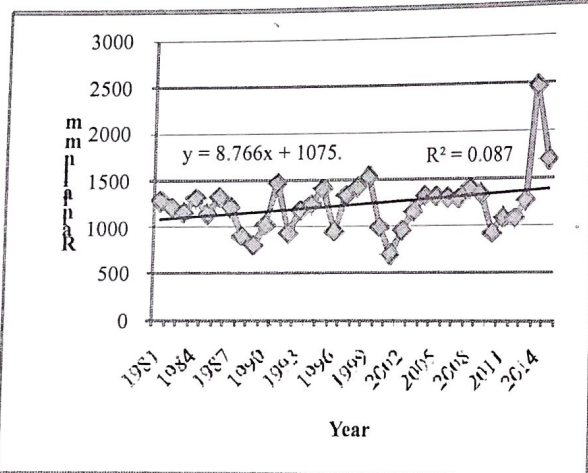
Figure 4: Annual rainfall over Ilorin, 1981–2015 Figure 5: Annual rainfall over Jos, 1981–2015 Source: Authors' computation, 2018 Source: Authors' computation, 2018
