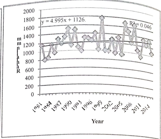
Figure 2: Annual rainfall over Makurdi, 1981–2015 Figure 3: Annual rainfall over Lokoja, 1981–2015 Source: Authors' computation, 2018 Source: Authors' computation, 2018
