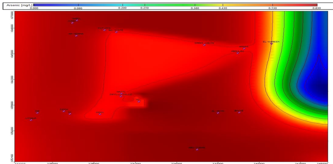
Figure 4: Predicted Arsenic Concentration after 1095 Days
