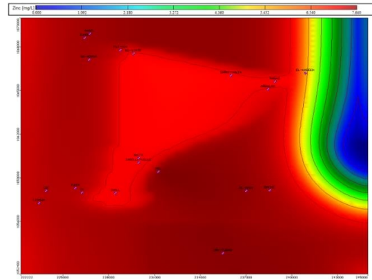
Figure 10: Concentration of Zinc after 1095 Days
