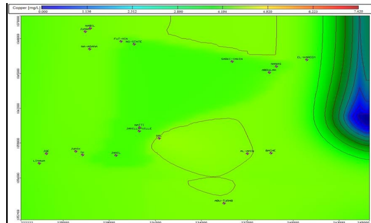
Figure 8: Predicted Copper Concentration after 1825 Days
