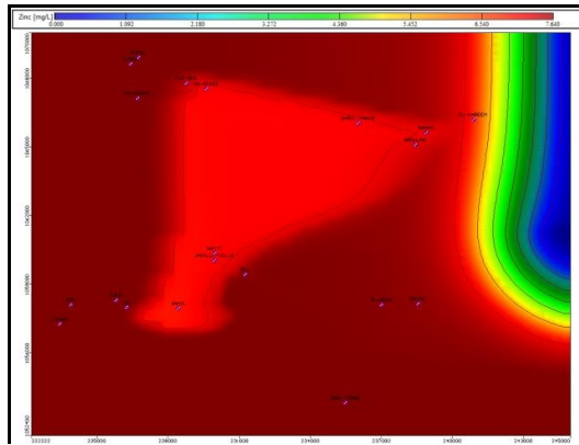
Figure 9: Concentration of Zinc after 365 Days
