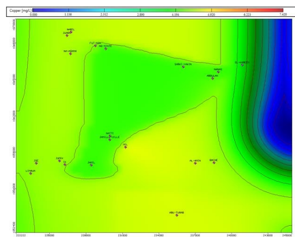
Figure 7: Predicted Copper Concentration after 1095 Days
