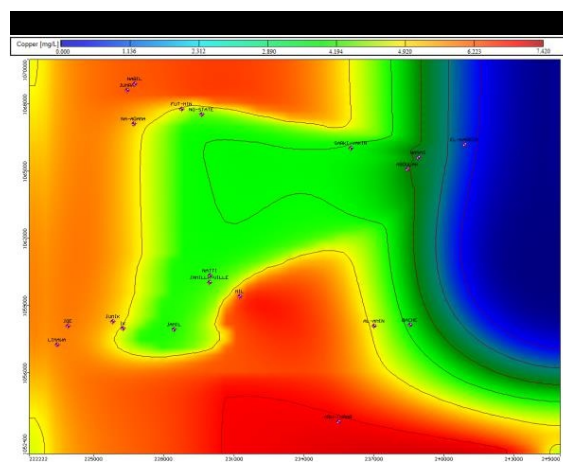
Figure 6: Predicted Copper Concentration after 365 Days
