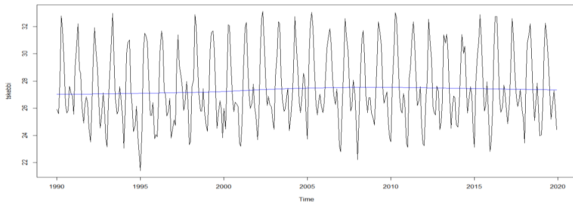
Fig. 2a. Time plot of the time series observation of Birnin Kebbi in Nigeria against months for the period 1990 – 2019
