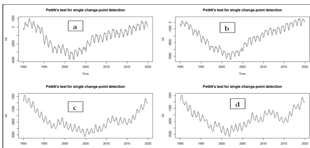
Fig. 7. Pettitt's test for single change-point detection in maximum temperature for Birnin Kebbi (a), Kano (b), Ibadan (c) and Owerri (d) for the period 1990-2019
