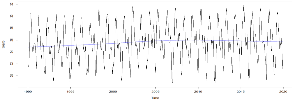
Fig. 2b. Time plot of the time series observation of Kano in Nigeria against Months for the period 1990 – 2019
