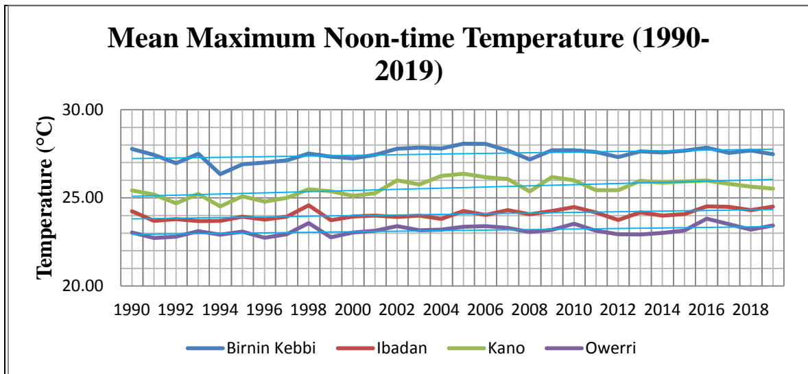
Fig. 5. Annual temperature trends across the four cities from 1990-2019
