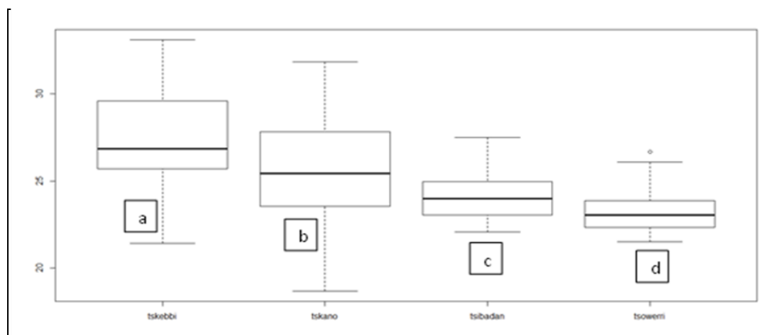
Fig. 3. Box plots of Maximum Noon-time temperature against time for Birnin Kebbi (a), Kano (b), Ibadan (c) and Owerri (d)
