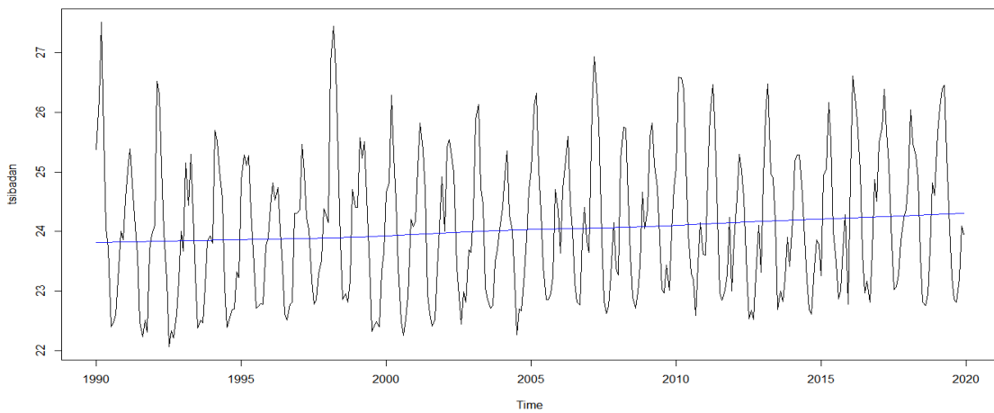
Fig. 2c. Time plot of the time series observation of Ibadan in Nigeria against months for the period 1990 – 2019
