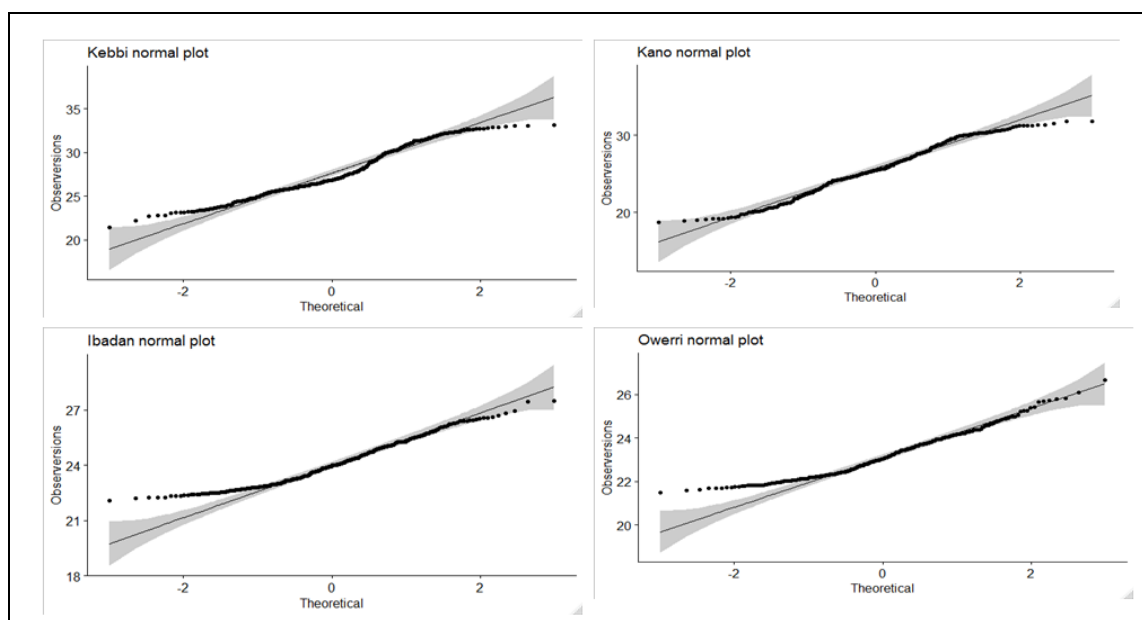
Fig. 4. Normal probability plot of maximum noon-time temperature for Birnin Kebbi, Kano, Ibadan and Owerri
