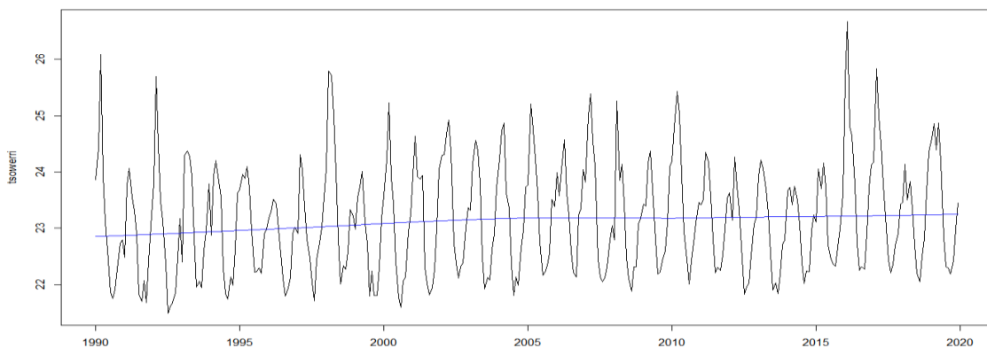
Fig. 2d. Time plot of the time series observation of Owerri in Nigeria against months for the period 1990 – 2019
