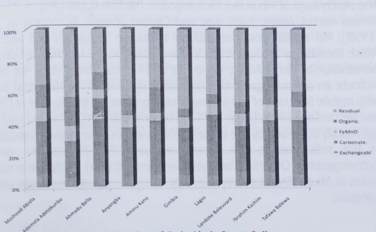
Figure 2: Chemical Fractionation of Cu in Abuja Street Soils
