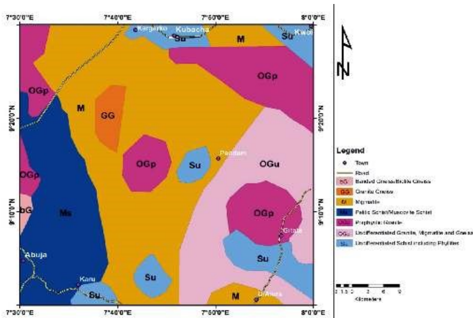
Fig. 3 Geologic Map of the Area
