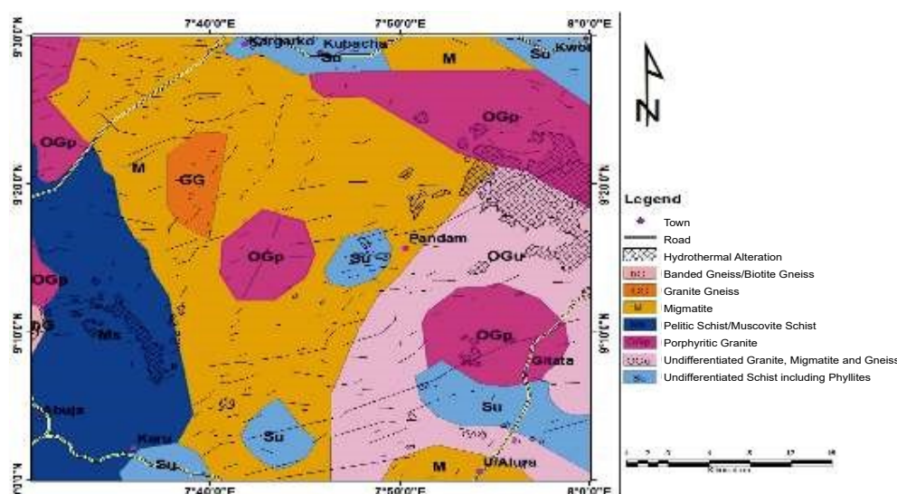
Fig. 11 Composite Proposed Geologic Map of the Area
