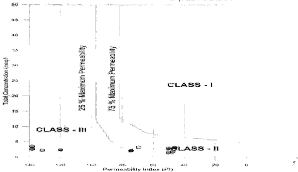
Figure 5. Doneen's Chart for Permeability Index for the study area.
