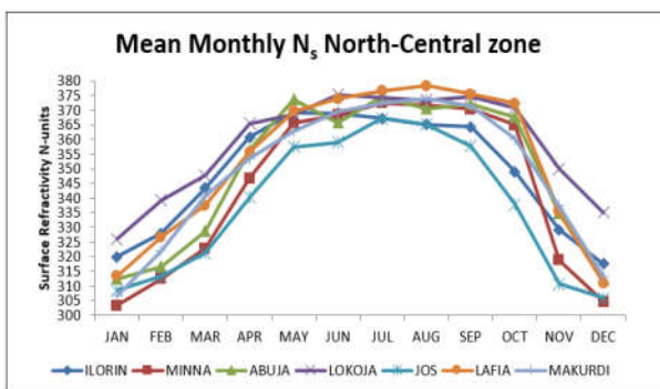
Fig. 9 Mean Monthly Surface Refractivity ( N_s ) over the North-central Stations for (2005-2010)
