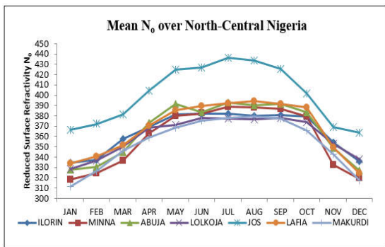
Fig. 12 Mean Monthly Reduced to-sea-level Refractivity N_0 for the seven stations between 2005-2010
