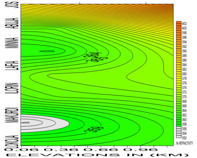
Fig. 13 2-D contour of mean yearly N_0 with elevations for the seven stations 2005-2010
