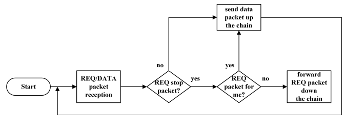
Fig. 2: LTDA-MAC network node operation.
