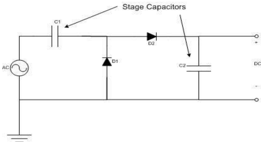
Fig. 7 Stage Capacitance
