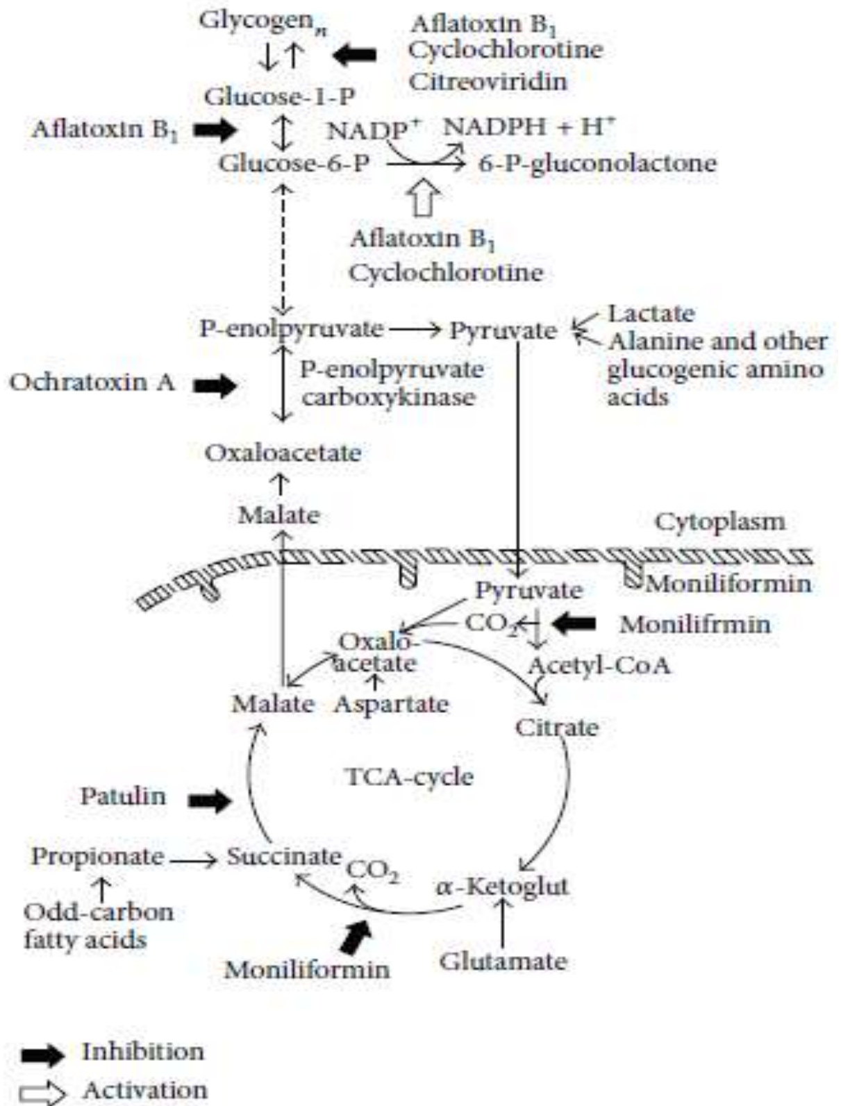
Fig 2.3: Inhibition of Oxidative Phosphorylation by Aflatoxins (Jimoh and Kolapo, 2018).
