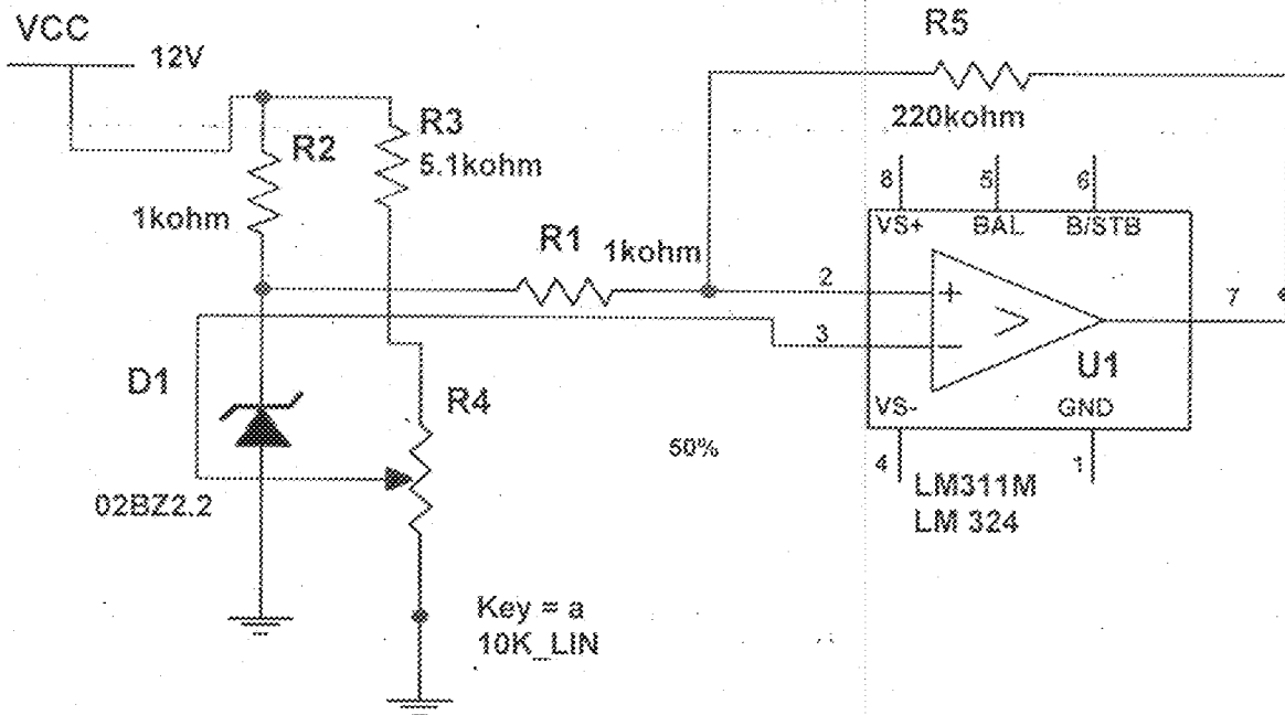
Voltage through the non-inverting input of comparator 1
