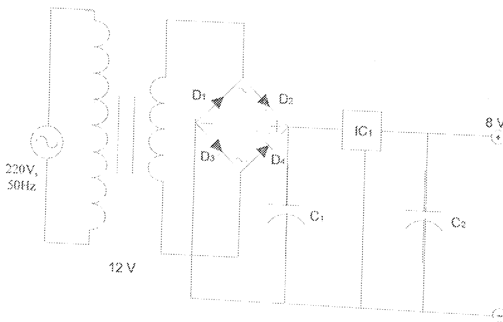
FIG 2.5 THE POWER UNIT
