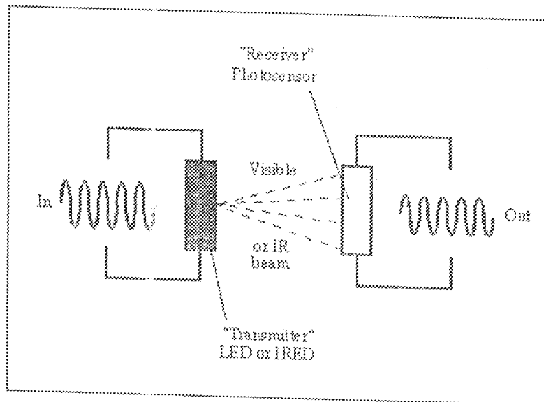
FIG 2.0 OPTOISOLATOR
