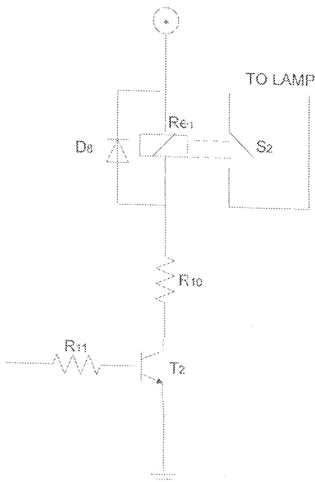
FIG. 2.4 THE AUTO SWITCH CIRCUIT
