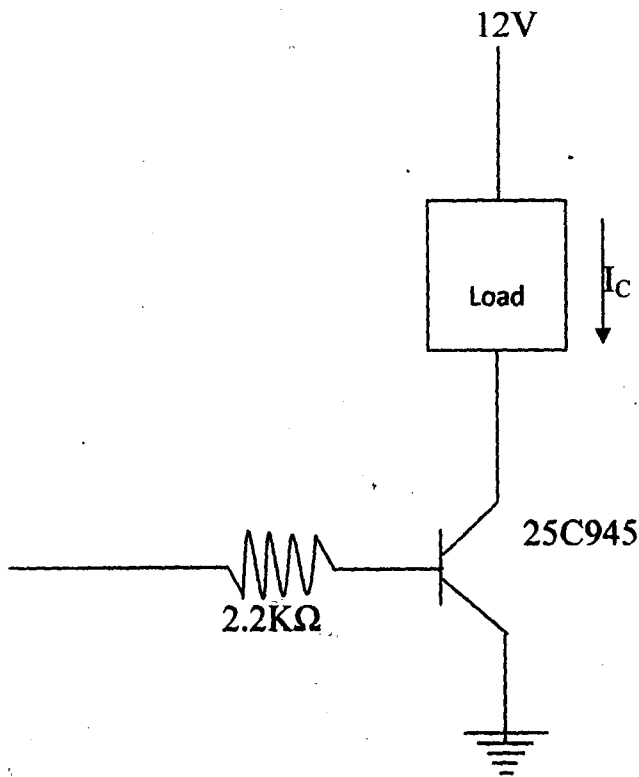
Fig 3.11 transistor circuit
