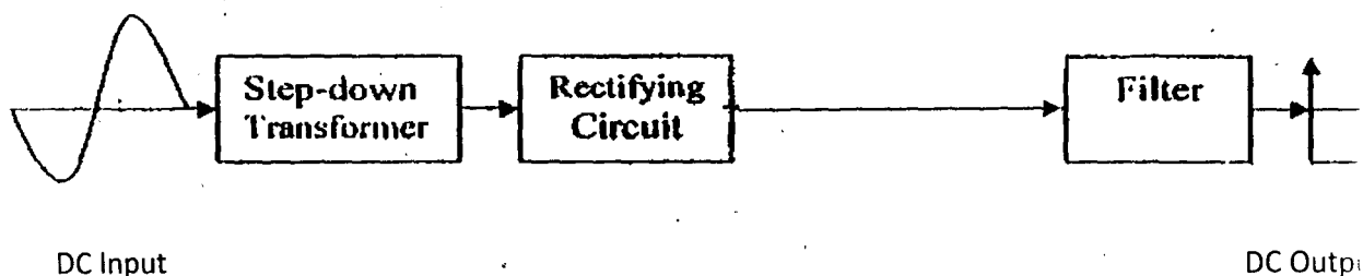
fig.2.1 lock Diagram of the Regulated Power Supply.
