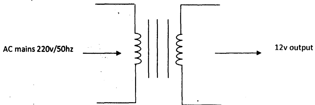
Fig 3.3 Transformer
