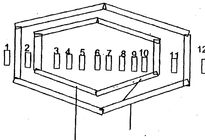
Fig. 3.7: When two coils are placed in slot
