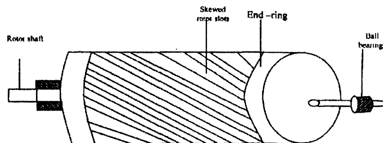
Fig 2.2: Rotor of an induction motor
