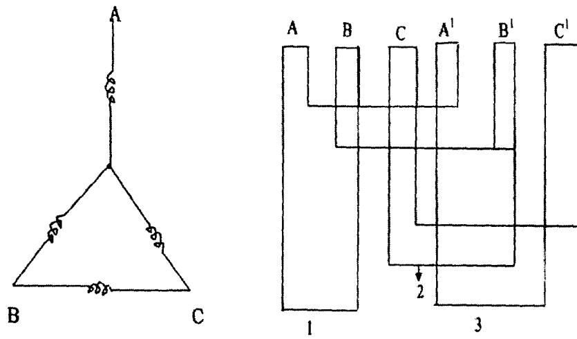
Fig 3.10 Delta Connection
