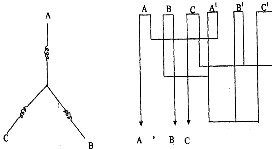
Fig 3.9 Star Connection
