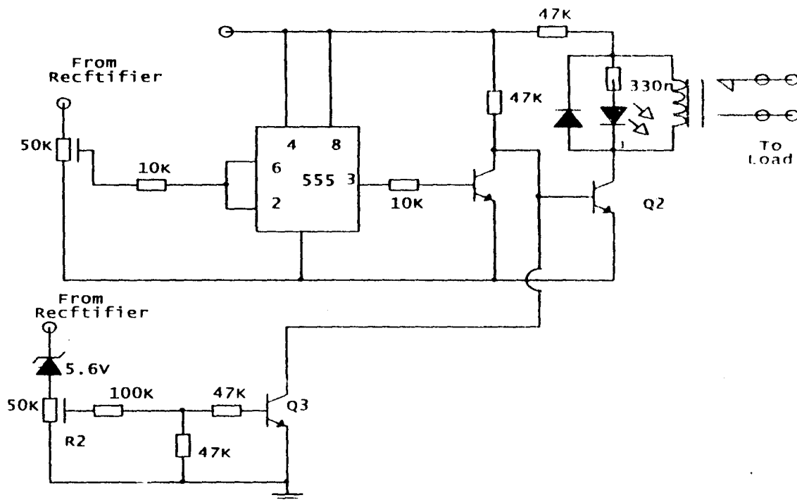
Fig. 3.1 under voltage / over voltage Detector
