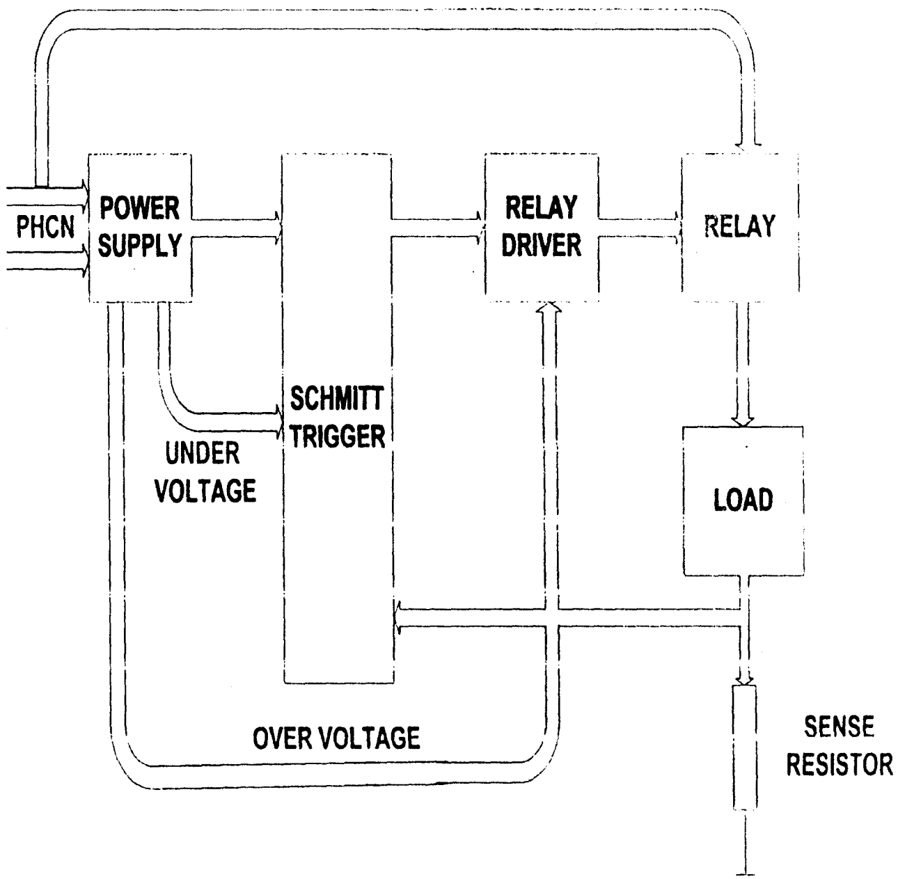
Fig. 2.4 Block Diagram
