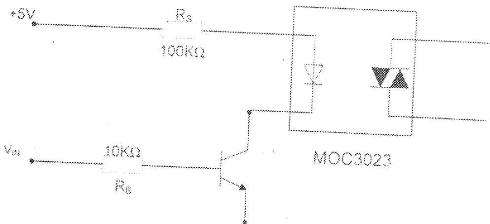
Fig 3.5 TRANSISTOR-OPTO-TRIAC SWITCH
