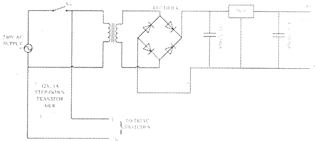
FIG 3.2 Power supply unit
