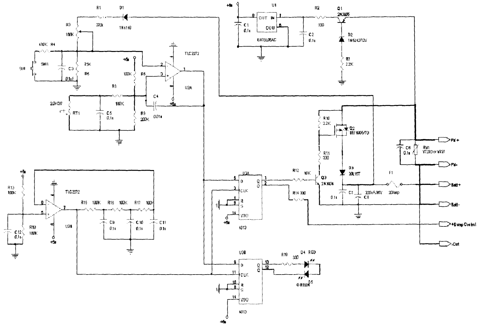
SOLAR CHARGE CONTROLLER CIRCUIT DIAGRAM
