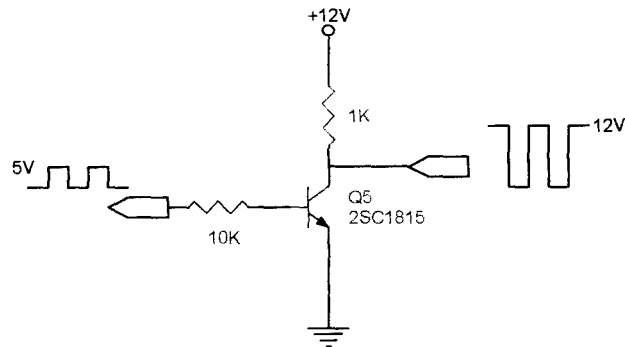
Fig 3.2.2 Field effect drive circuit
