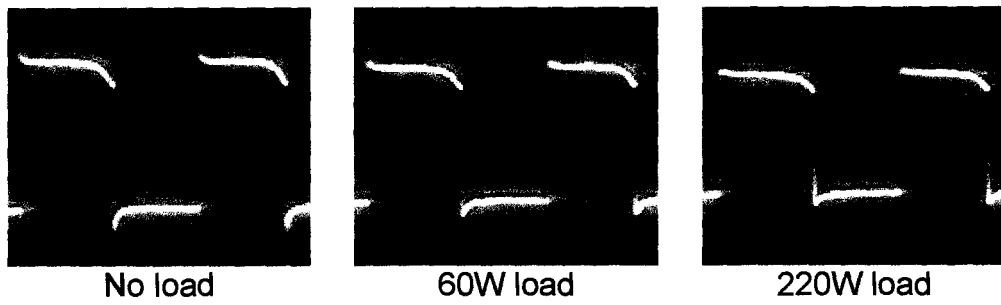
Plate 4.4.2 The output signal waveform
