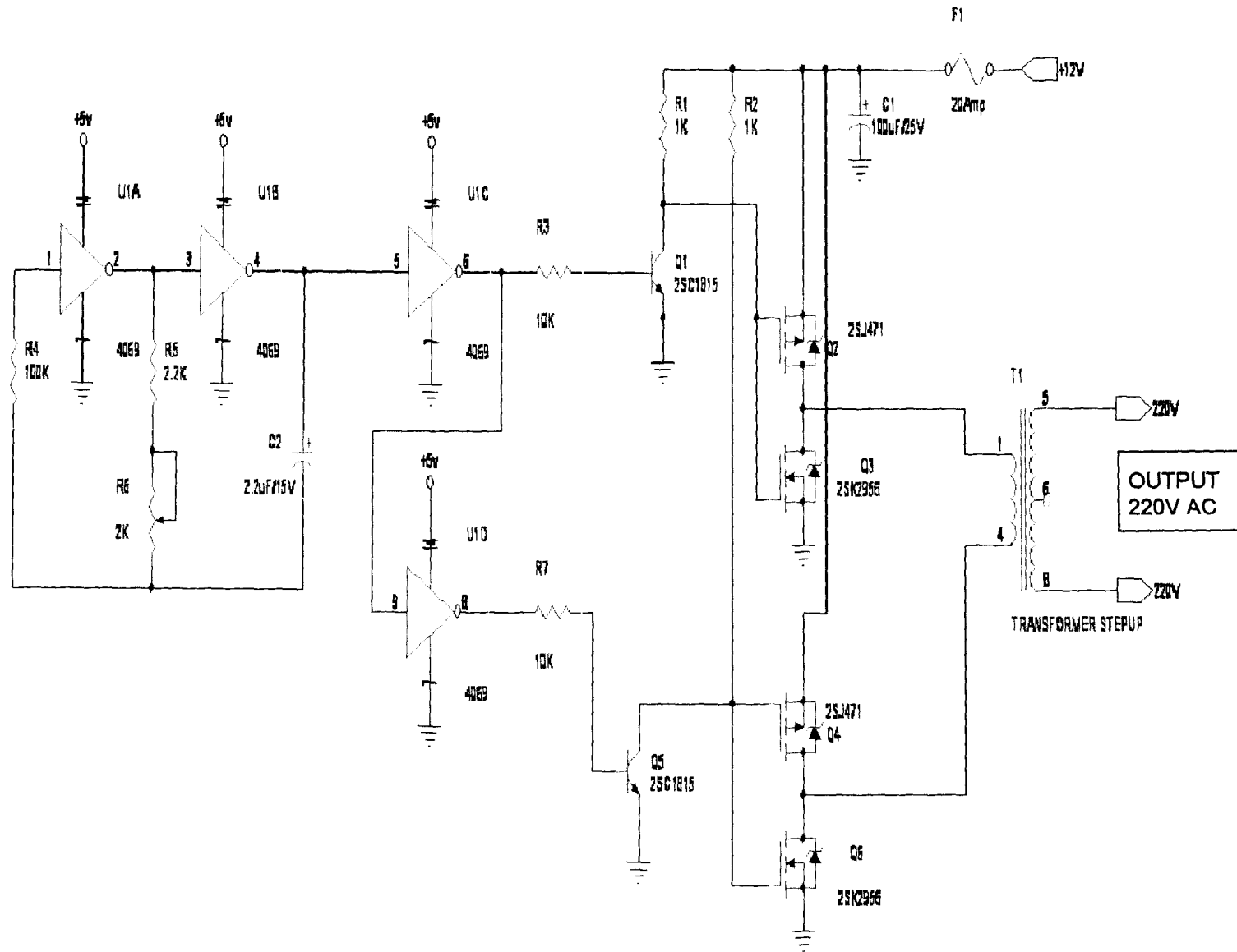
INVERTER CIRCUIT
