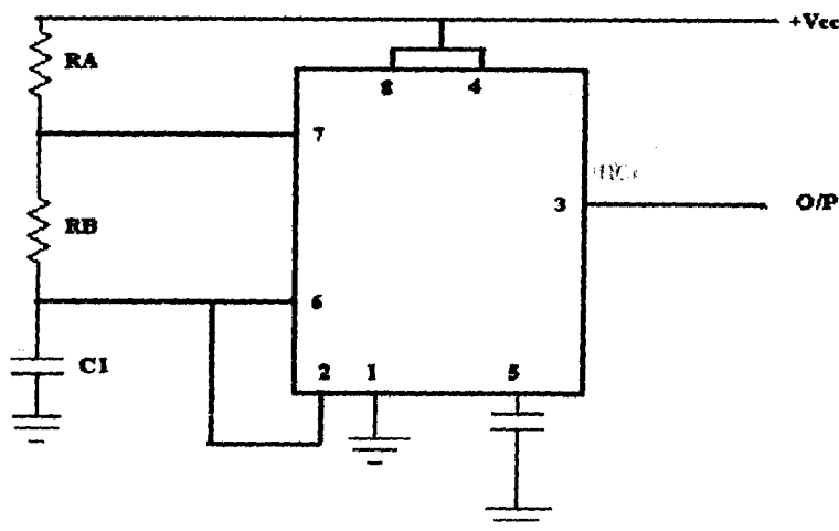
Fig 3.7 Astable mode
