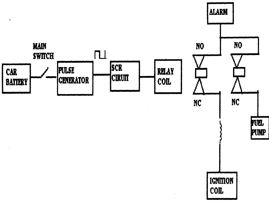
BLOCK DIAGRAM FOR THE AUTOMATIC CAR DEMOBILIZER
