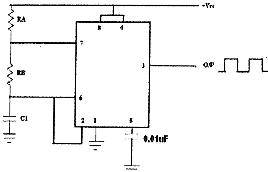
Figure 3.3a 555 Timer IC
