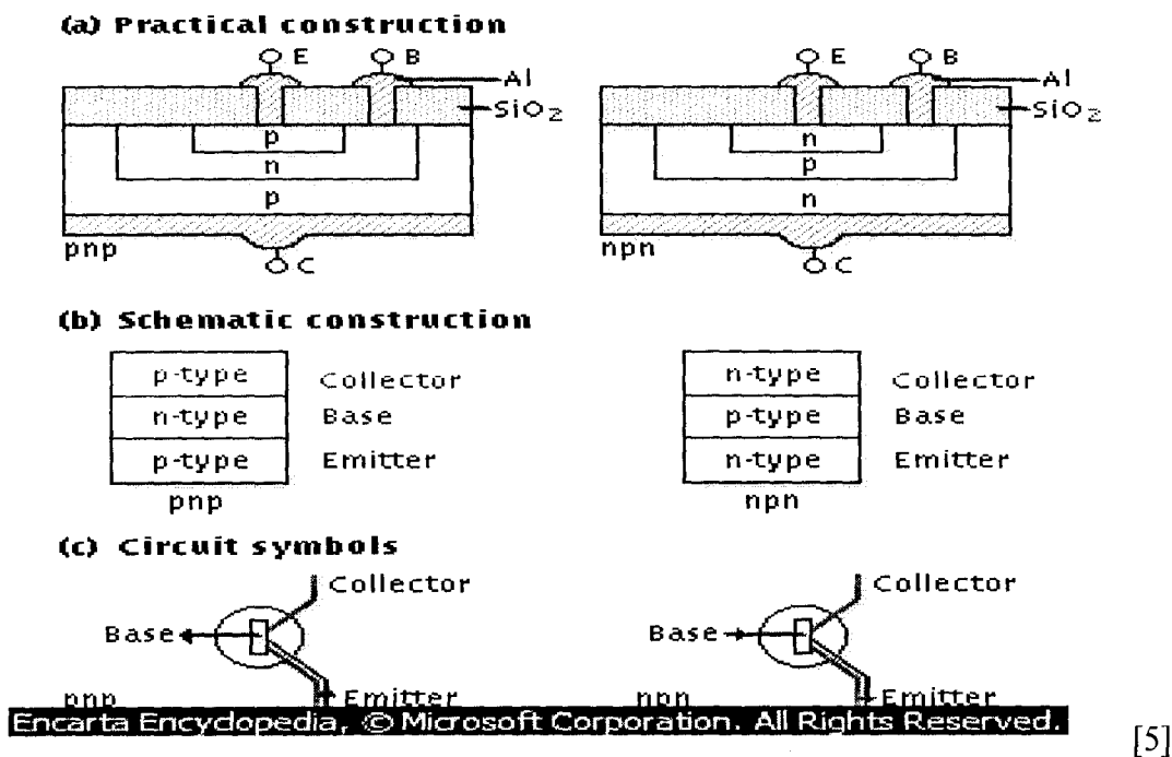
Figure 2.2 the practical, schematic and symbolic transistor diagram
