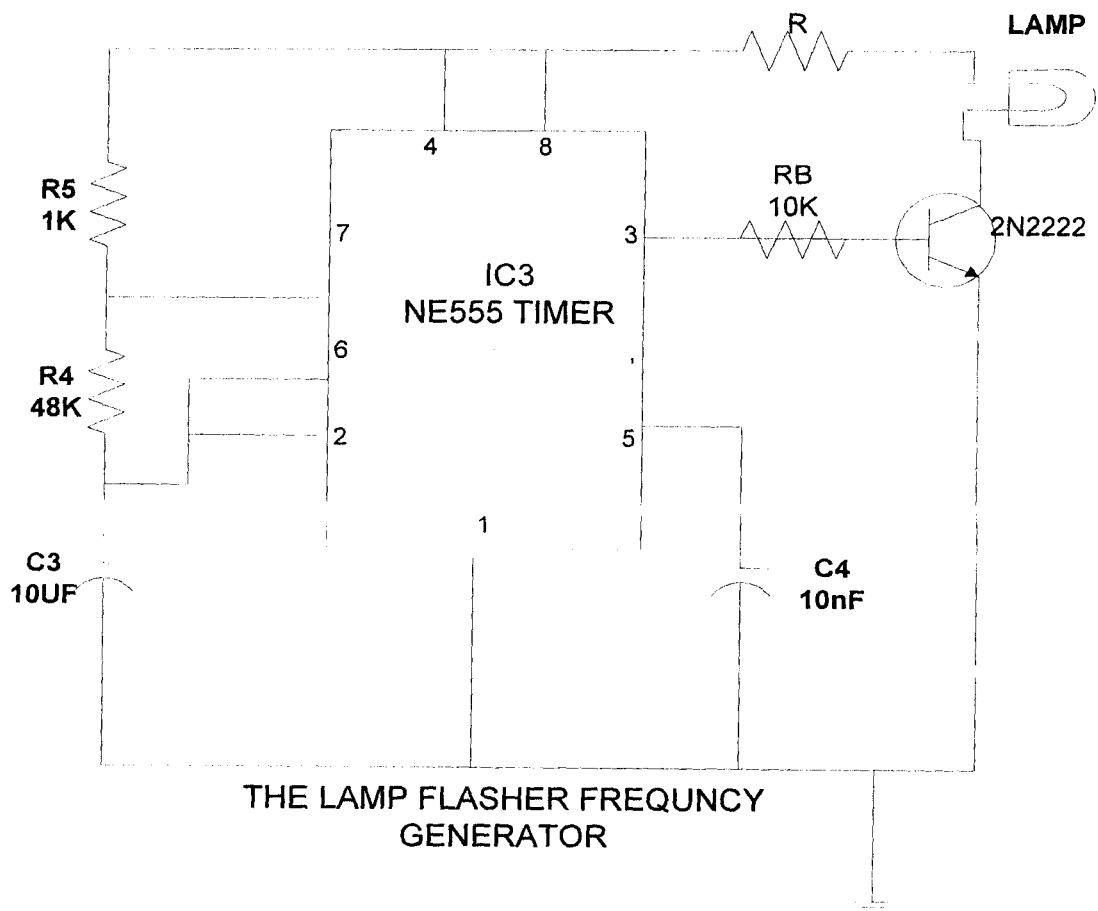
Figure 3.8 the lamp flasher unit.
