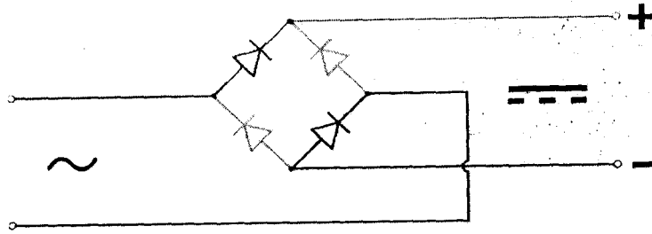
Figure 3.4 positive conventional of current in a full bridge rectifier.
