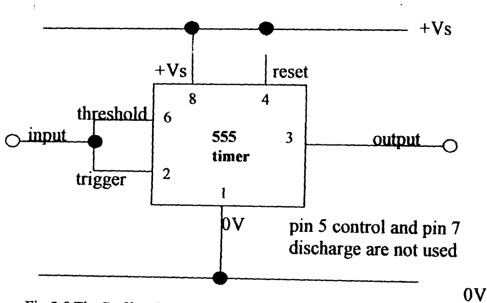
Fig 2.8 The Buffer circuit of 555 timer
