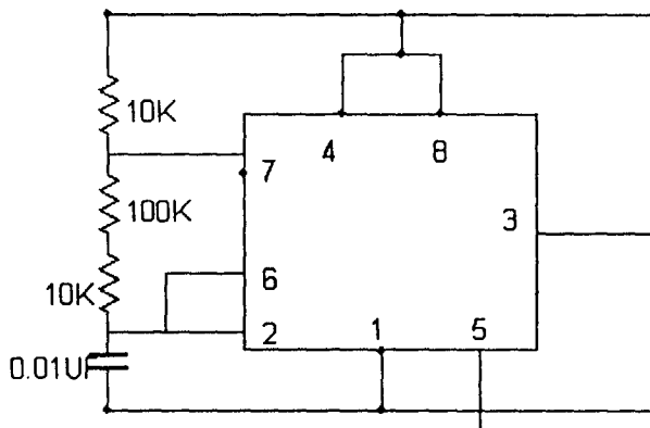
Fig 3.4b Oscillator circuit for the second 555 timer
