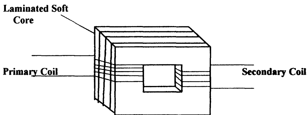
Fig 2.3a A Step down Transformer
