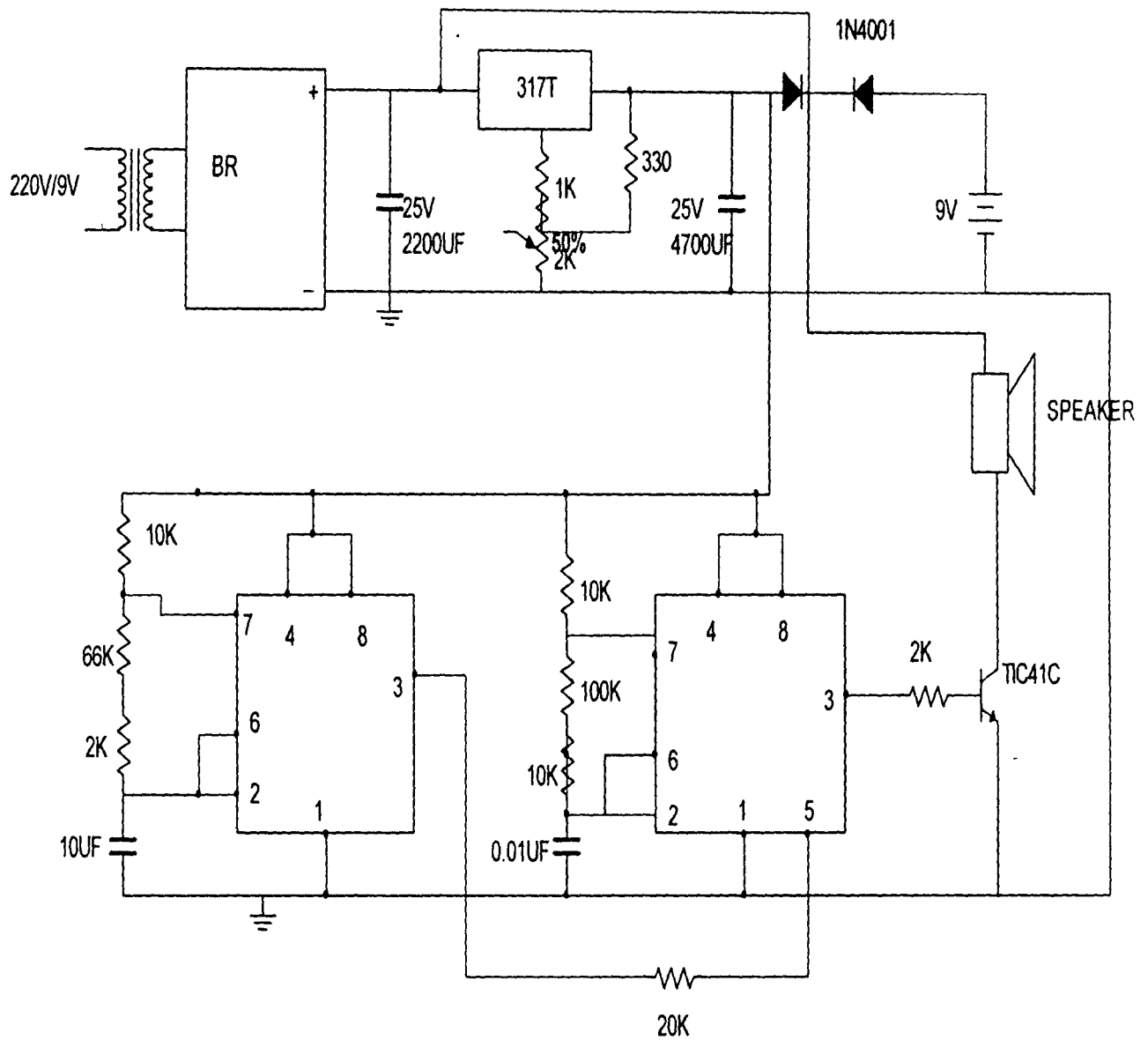
Fig 3.5 The Circuit Diagram of an Ambulance Siren
