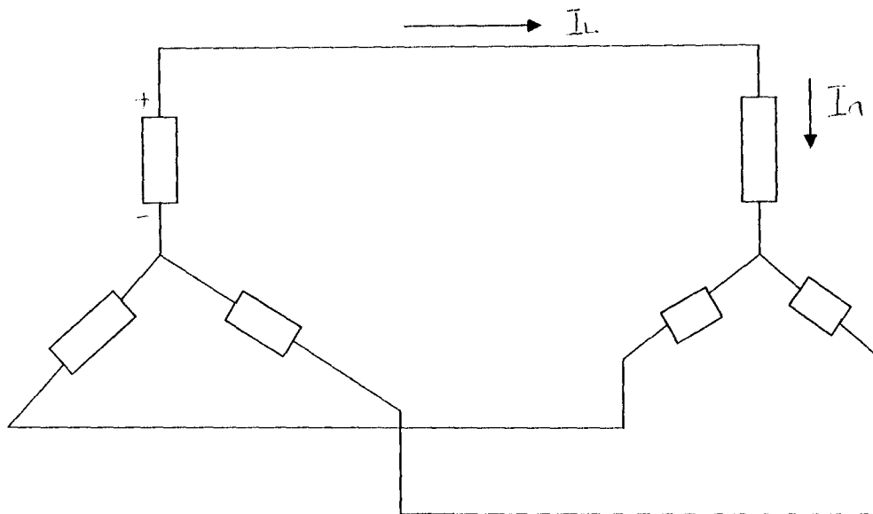
Fig 2.1: star-star connection
