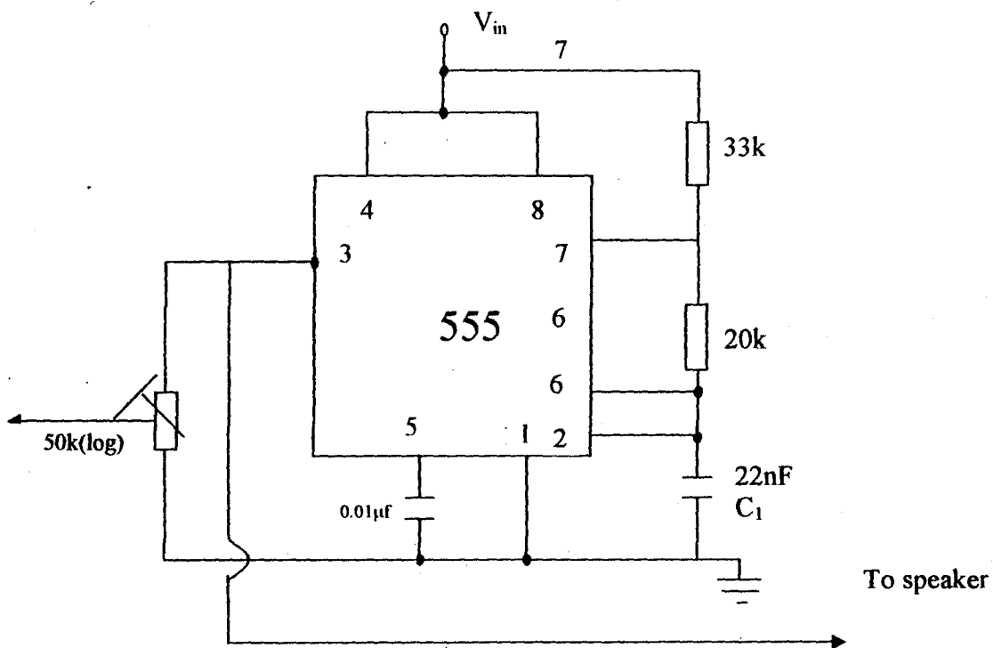
Fig. 3.12 Tone generator
