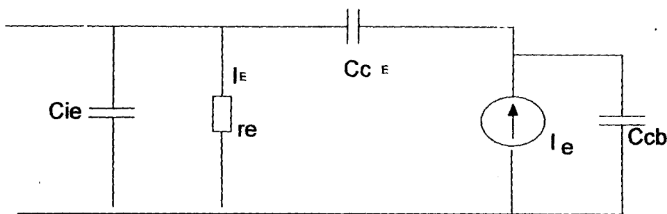
Fig. 3.22 Tuned collector stage
