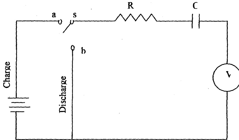
Fig. 3.14 Capacitor charging/ discharging circuit
