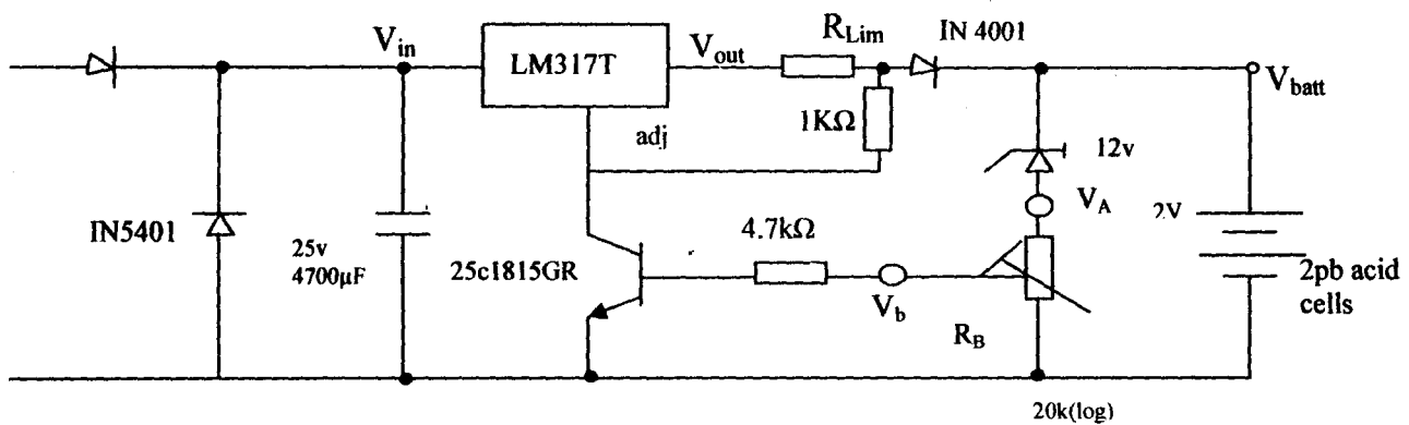
Fig 3.9: Charging unit
