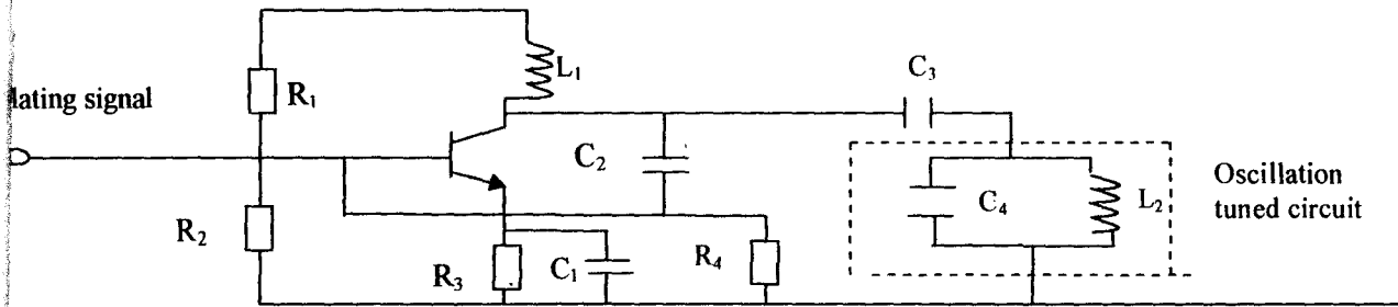
Fig 3.20 Transistor reactance modulator
