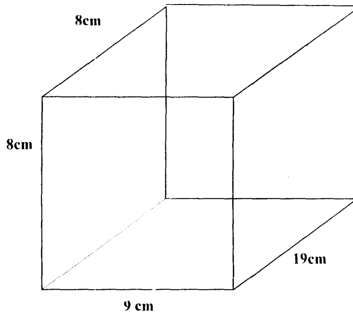
Figure 4.1: Casing dimension
