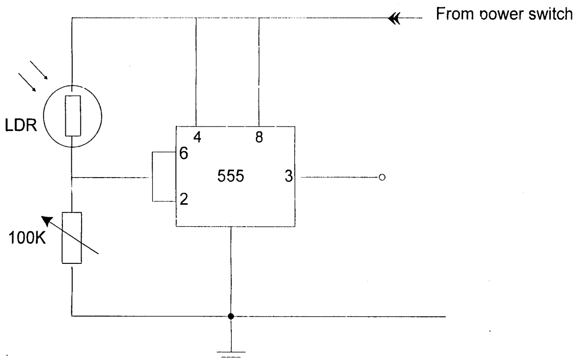
Fig 3.5 555 Schmitt Trigger
