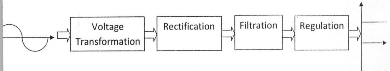
Fig 2.2: Power Unit
