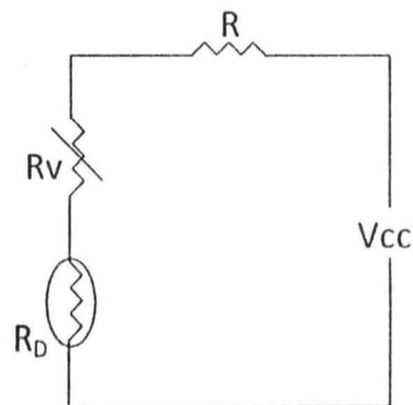
Fig 3.2b: Equivalent Circuit
