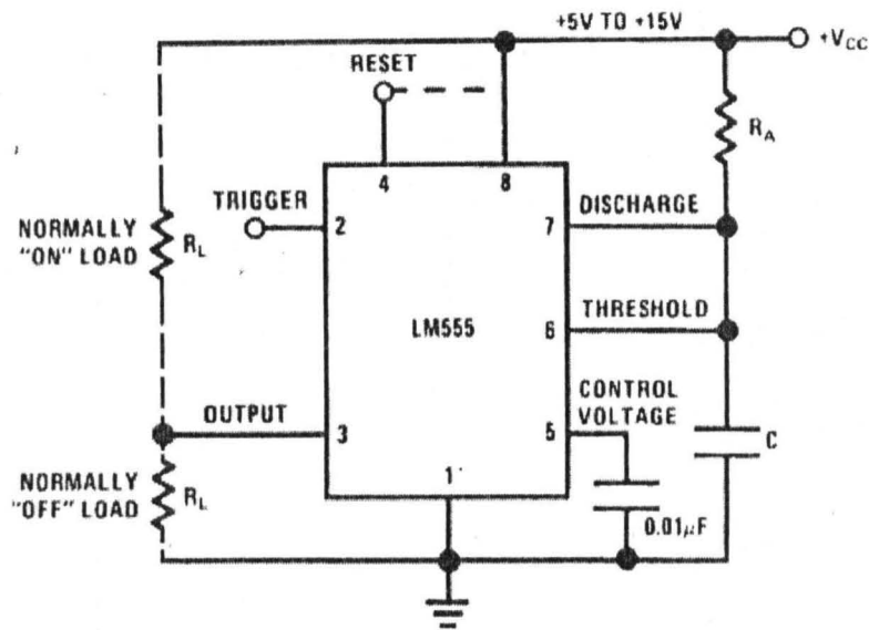
Fig 2.6: Monostable Configuration
