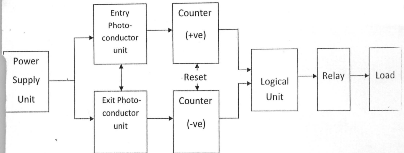
Fig 3.1: Block Diagram an automatic light switch
