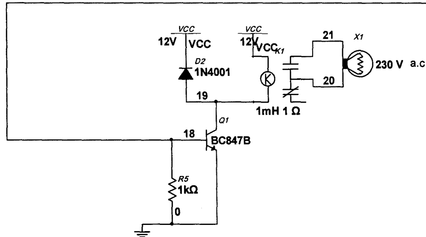
Figure: 4.0 A COMPLETE CIRCUIT DIAGRAM OF AN AUTOMATIC ROOM CONTROLLED HEATING SYSTEM
