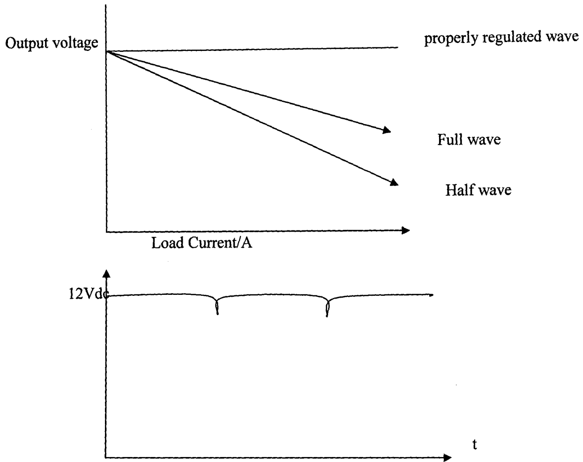
Fig 3.6 wave forms of regulated voltage output
