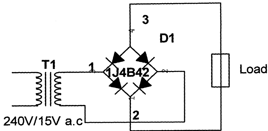
Fig. 3.3 Schematic diagram of rectifier circuit
