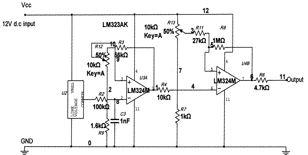
Fig: 3.8 Schematic diagram of a sensing circuit
