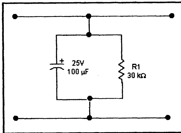
Fig.3.7.3a Filter circuit
