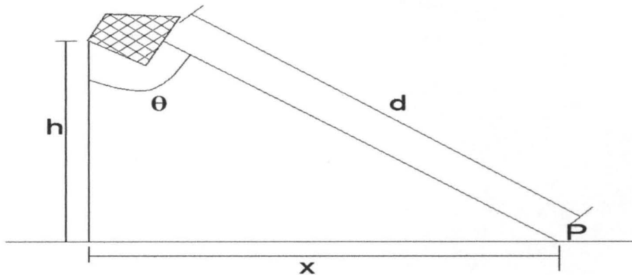
Fig. 3.1 the required dimensions to determine illumination at point P
