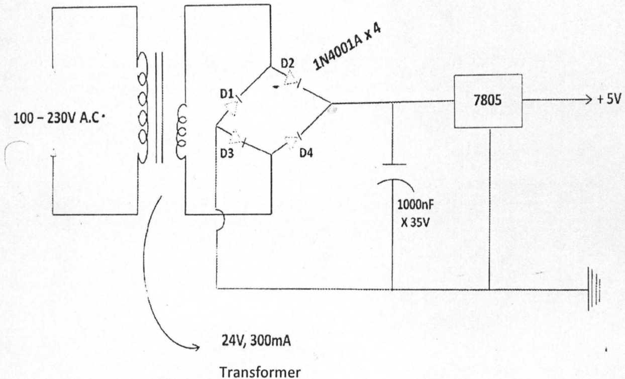
Fig 3.3 Circuit Diagram of Power Supply Unit
