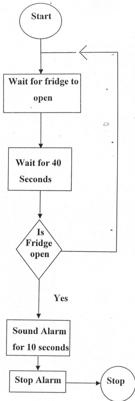
Fig 3.6 Flow Chart of Entire Program
