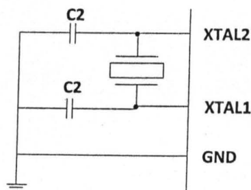
Figure 3.4 Oscilalator connection
