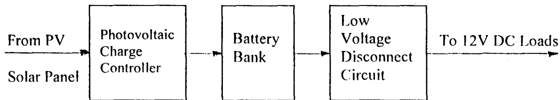
Figure 3.0 12V Solar Power Centre Block diagram
